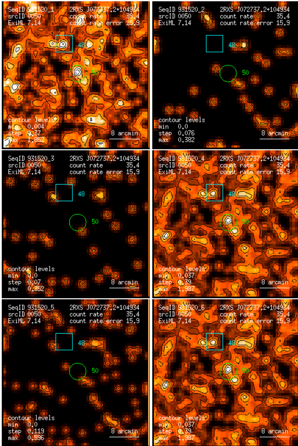
Figure 50: RASS 931520: detection 0050: band rate images, Gaussian filter: (1) PSPC channels 11 – 41, (2) 52 – 90, (3) 91 – 201, (4) 11 – 235, (5) 52 – 201, (6) 11 – 201. Broad band rates in counts/ks. Band rate contour levels in counts/ks/arcmin 2 .
