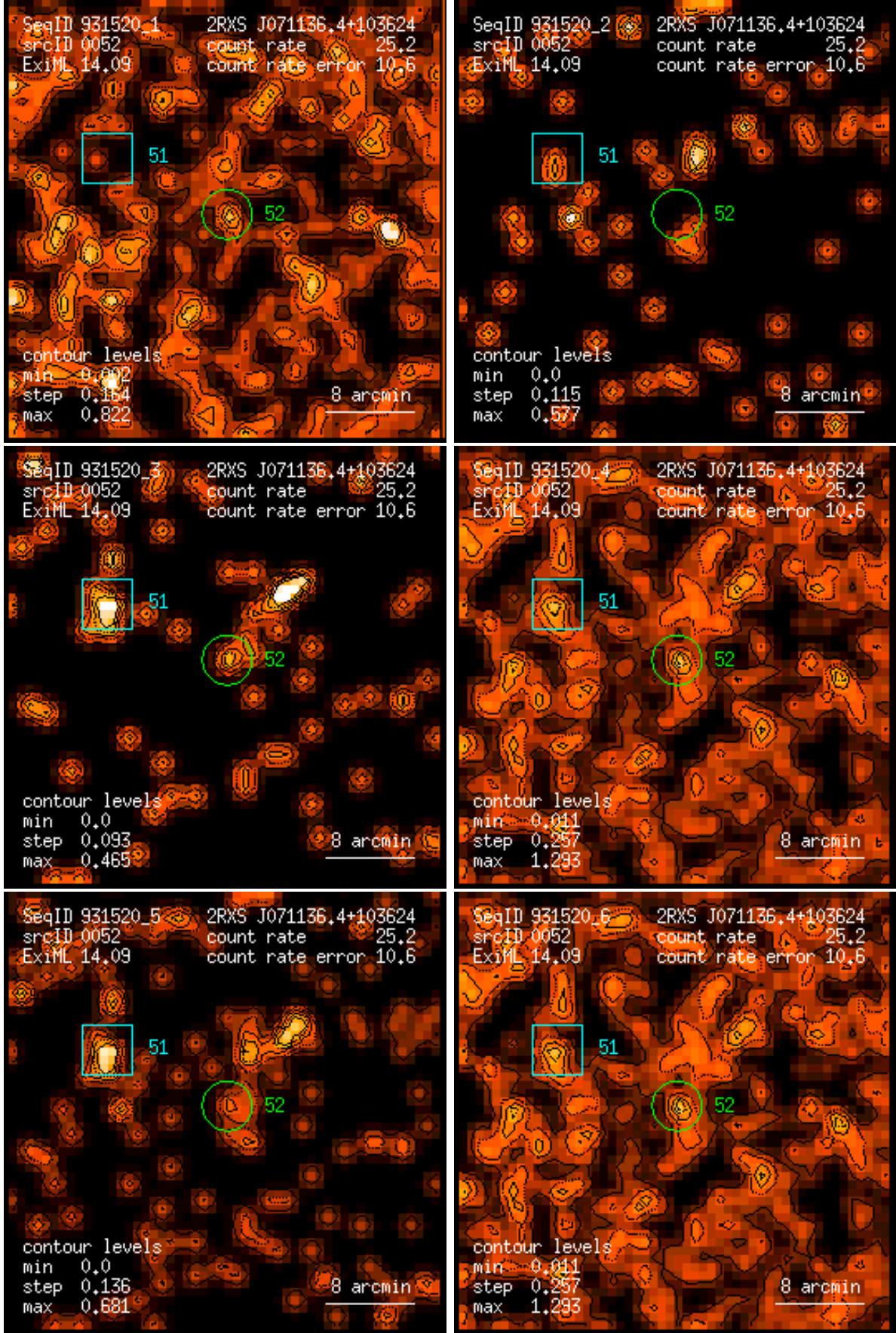
Figure 52: RASS 931520: detection 0052: band rate images, Gaussian filter: (1) PSPC channels 11 – 41, (2) 52 – 90, (3) 91 – 201, (4) 11 – 235, (5) 52 – 201, (6) 11 – 201. Broad band rates in counts/ks. Band rate contour levels in counts/ks/arcmin 2 .
