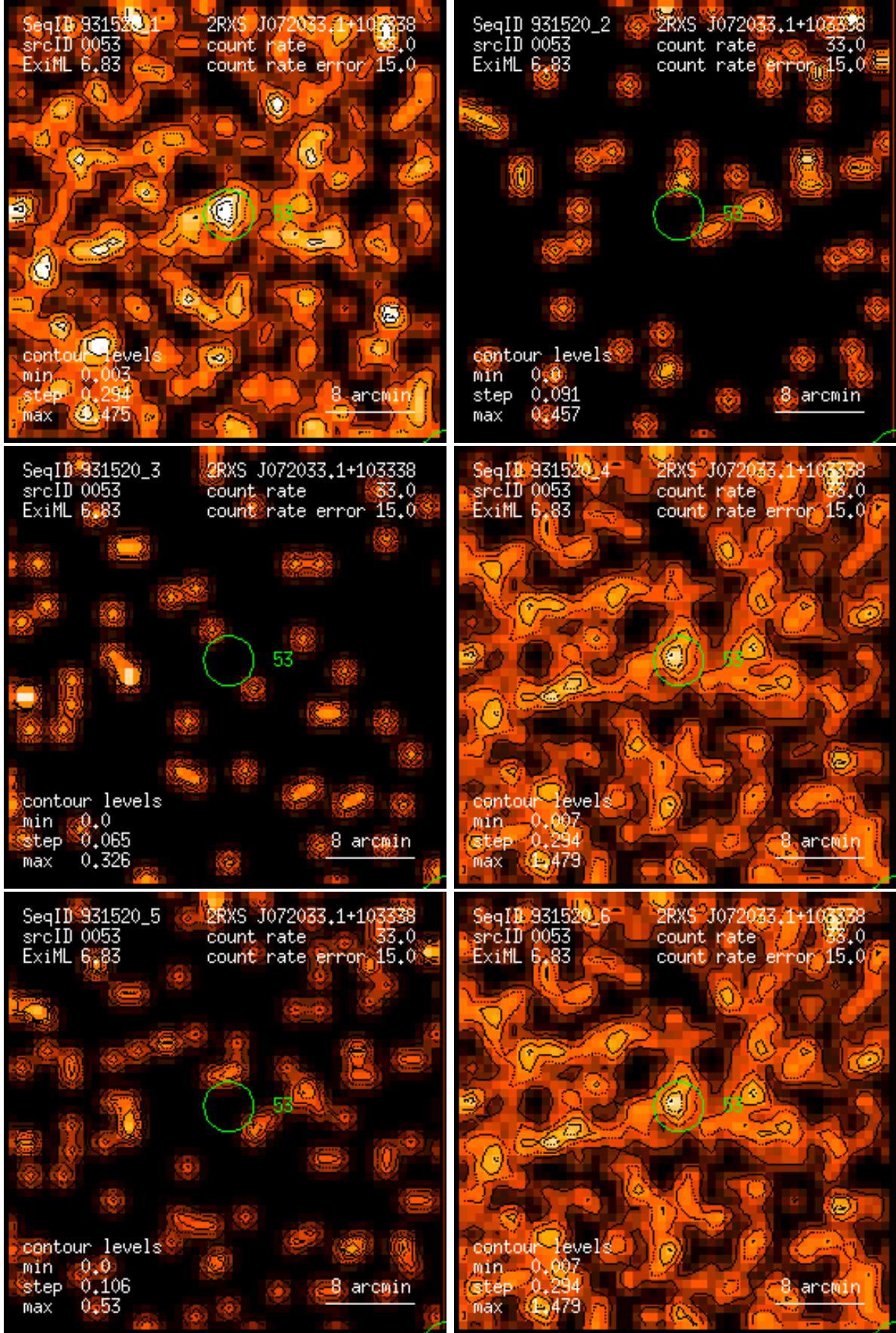
Figure 53: RASS 931520: detection 0053: band rate images, Gaussian filter: (1) PSPC channels 11 – 41, (2) 52 – 90, (3) 91 – 201, (4) 11 – 235, (5) 52 – 201, (6) 11 – 201. Broad band rates in counts/ks. Band rate contour levels in counts/ks/arcmin 2 .
