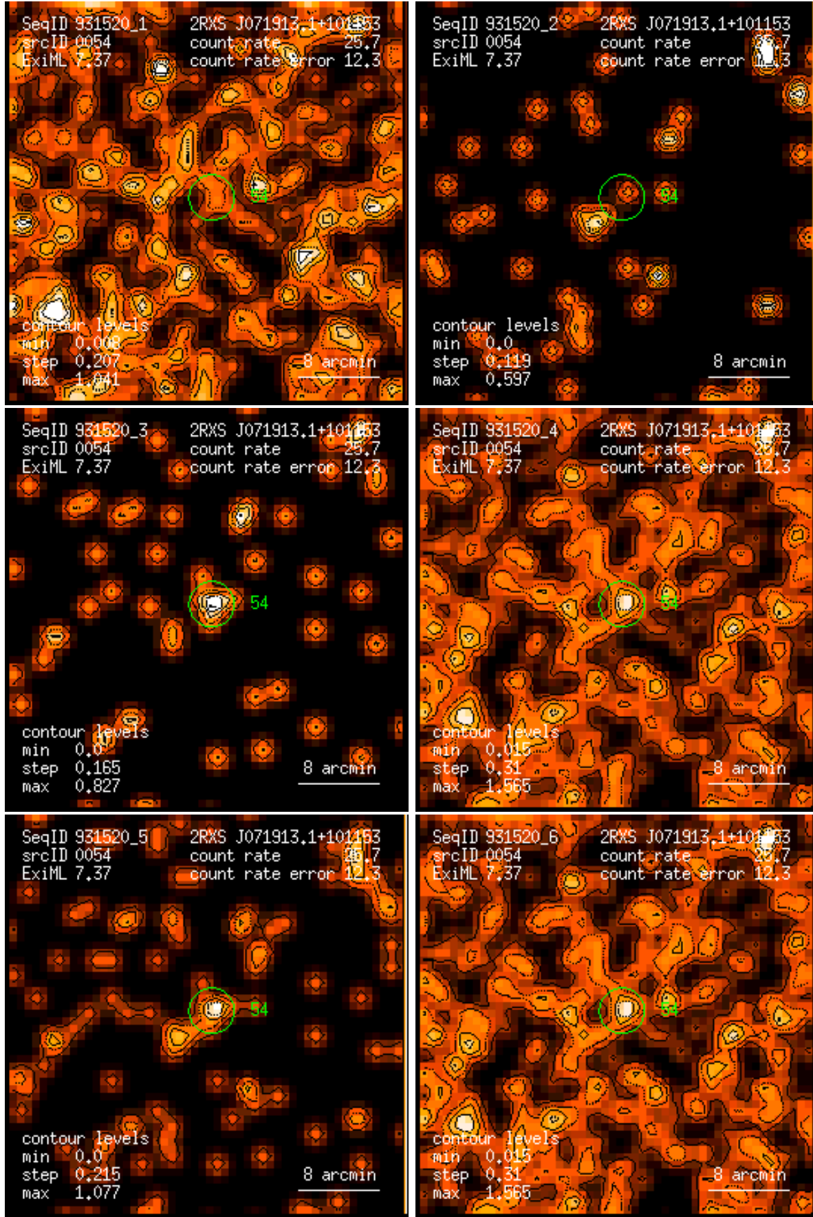
Figure 54: RASS 931520: detection 0054: band rate images, Gaussian filter: (1) PSPC channels 11 – 41, (2) 52 – 90, (3) 91 – 201, (4) 11 – 235, (5) 52 – 201, (6) 11 – 201. Broad band rates in counts/ks. Band rate contour levels in counts/ks/arcmin 2 .
