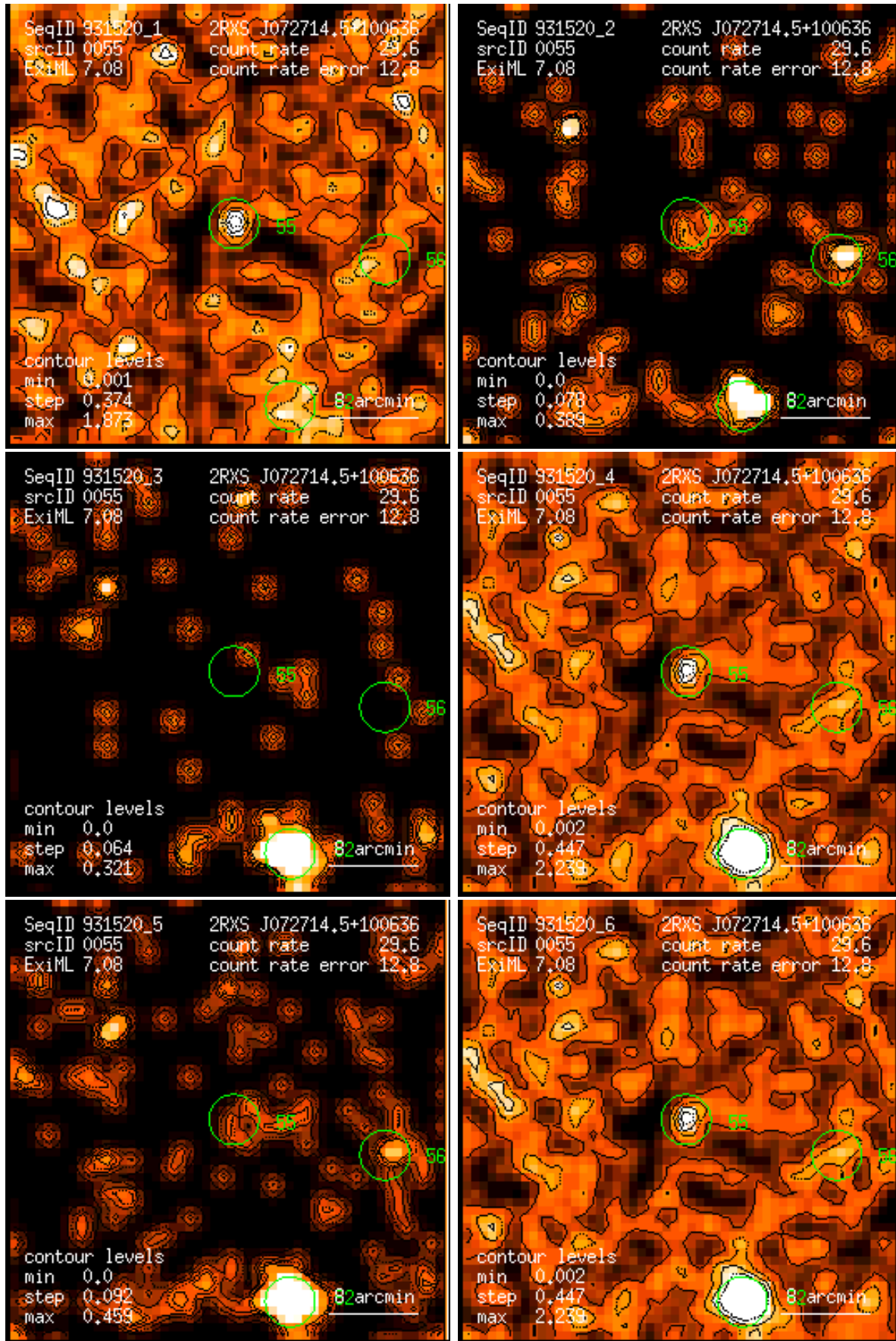
Figure 55: RASS 931520: detection 0055: band rate images, Gaussian filter: (1) PSPC channels 11 – 41, (2) 52 – 90, (3) 91 – 201, (4) 11 – 235, (5) 52 – 201, (6) 11 – 201. Broad band rates in counts/ks. Band rate contour levels in counts/ks/arcmin 2 .
