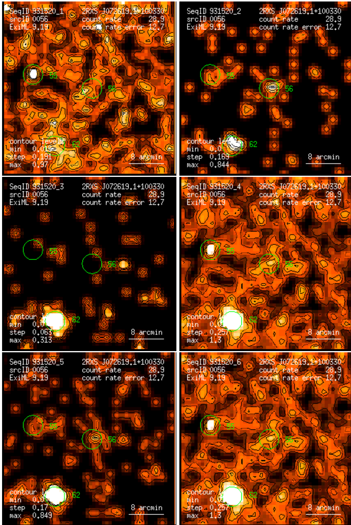
Figure 56: RASS 931520: detection 0056: band rate images, Gaussian filter: (1) PSPC channels 11 – 41, (2) 52 – 90, (3) 91 – 201, (4) 11 – 235, (5) 52 – 201, (6) 11 – 201. Broad band rates in counts/ks. Band rate contour levels in counts/ks/arcmin 2 .
