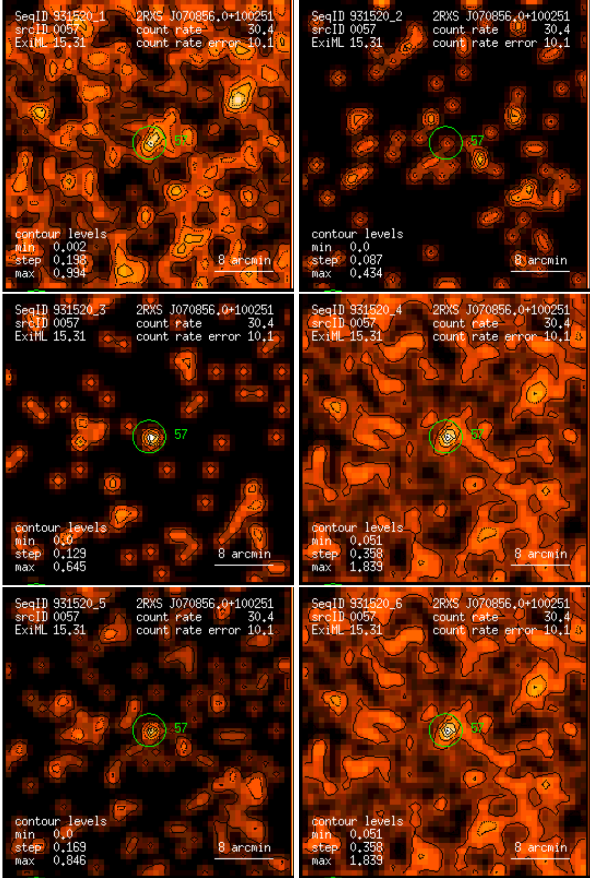
Figure 57: RASS 931520: detection 0057: band rate images, Gaussian filter: (1) PSPC channels 11 – 41, (2) 52 – 90, (3) 91 – 201, (4) 11 – 235, (5) 52 – 201, (6) 11 – 201. Broad band rates in counts/ks. Band rate contour levels in counts/ks/arcmin 2 .
