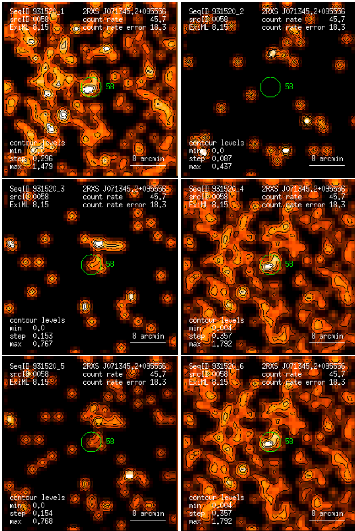
Figure 58: RASS 931520: detection 0058: band rate images, Gaussian filter: (1) PSPC channels 11 – 41, (2) 52 – 90, (3) 91 – 201, (4) 11 – 235, (5) 52 – 201, (6) 11 – 201. Broad band rates in counts/ks. Band rate contour levels in counts/ks/arcmin 2 .
