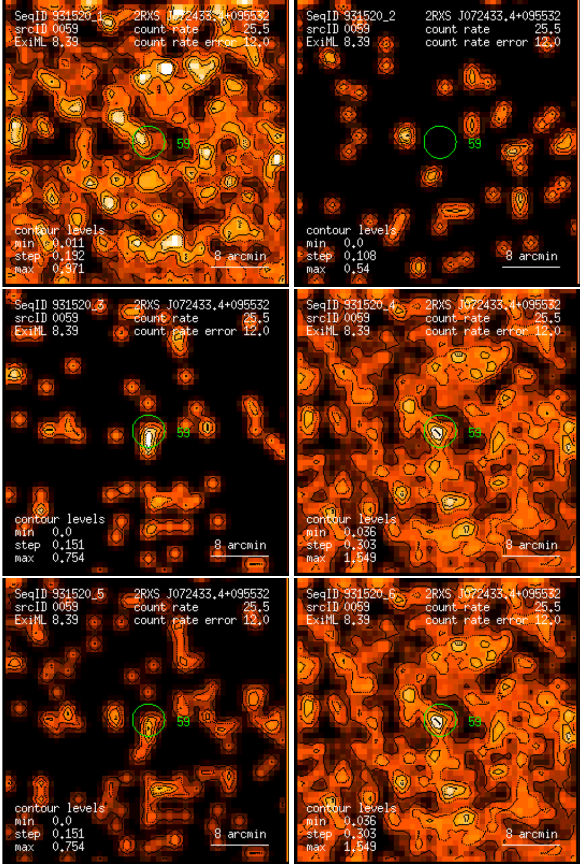
Figure 59: RASS 931520: detection 0059: band rate images, Gaussian filter: (1) PSPC channels 11 – 41, (2) 52 – 90, (3) 91 – 201, (4) 11 – 235, (5) 52 – 201, (6) 11 – 201. Broad band rates in counts/ks. Band rate contour levels in counts/ks/arcmin 2 .
