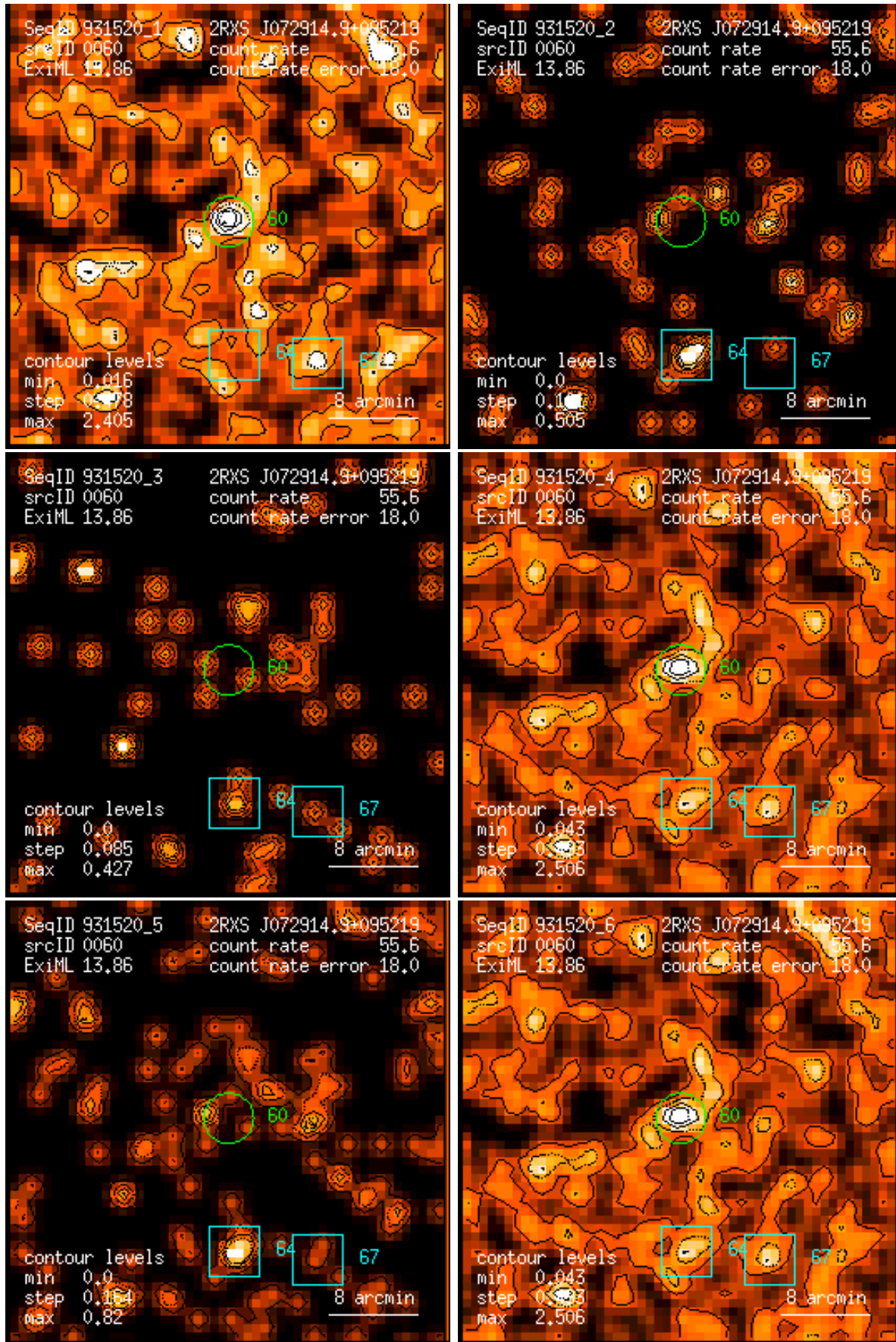
Figure 60: RASS 931520: detection 0060: band rate images, Gaussian filter: (1) PSPC channels 11 – 41, (2) 52 – 90, (3) 91 – 201, (4) 11 – 235, (5) 52 – 201, (6) 11 – 201. Broad band rates in counts/ks. Band rate contour levels in counts/ks/arcmin 2 .
