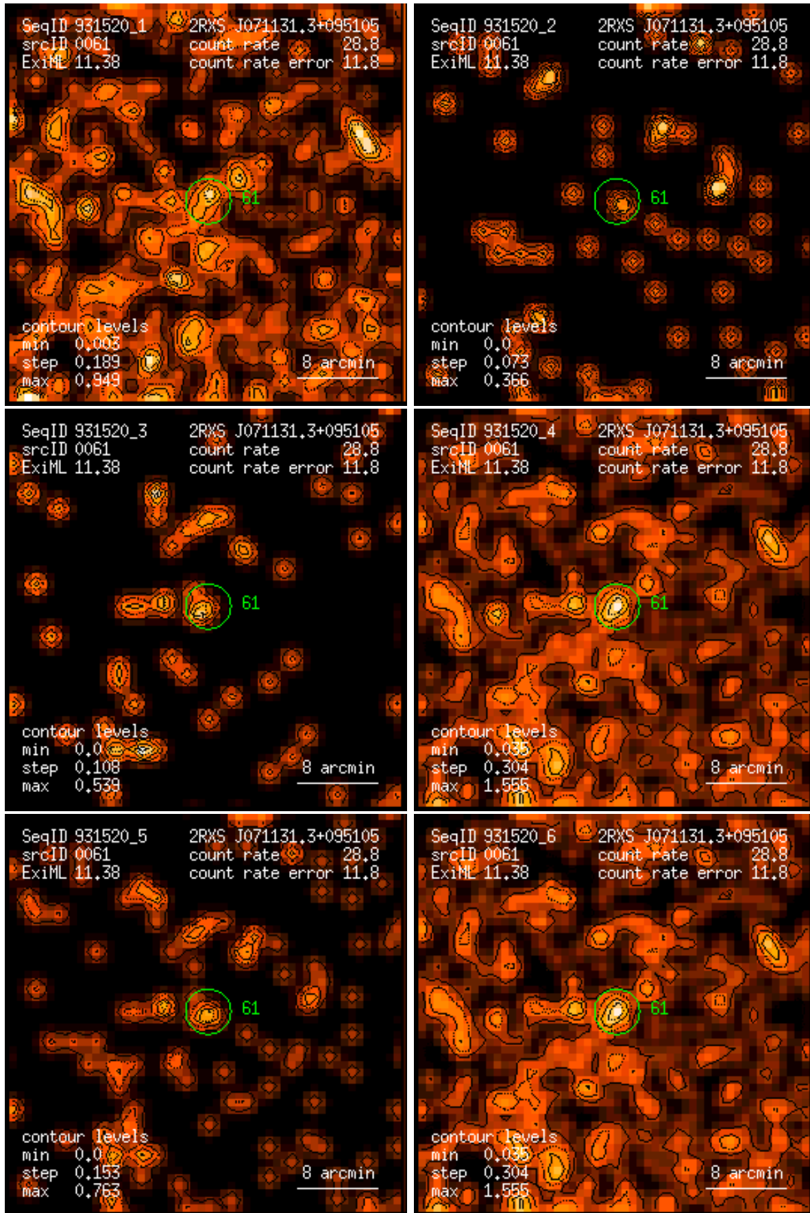
Figure 61: RASS 931520: detection 0061: band rate images, Gaussian filter: (1) PSPC channels 11 – 41, (2) 52 – 90, (3) 91 – 201, (4) 11 – 235, (5) 52 – 201, (6) 11 – 201. Broad band rates in counts/ks. Band rate contour levels in counts/ks/arcmin 2 .
