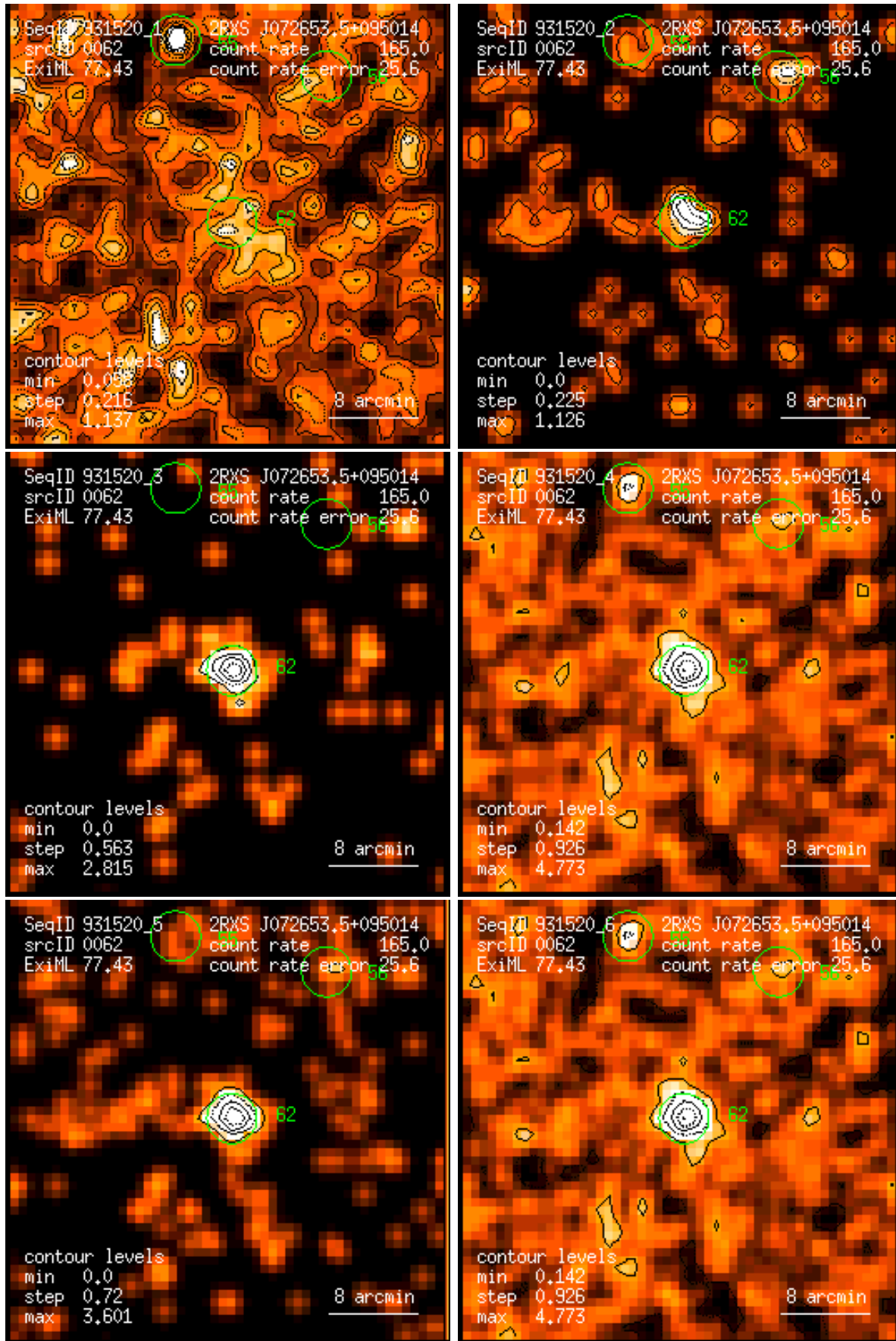
Figure 62: RASS 931520: detection 0062: band rate images, Gaussian filter: (1) PSPC channels 11 – 41, (2) 52 – 90, (3) 91 – 201, (4) 11 – 235, (5) 52 – 201, (6) 11 – 201. Broad band rates in counts/ks. Band rate contour levels in counts/ks/arcmin 2 .
