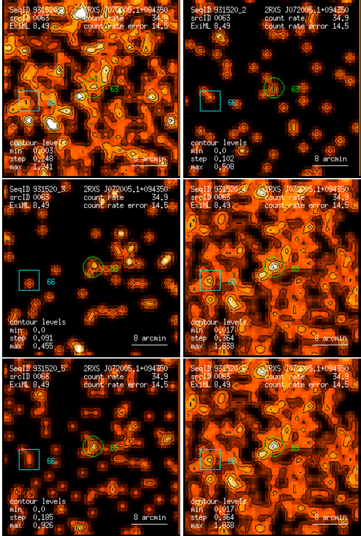
Figure 63: RASS 931520: detection 0063: band rate images, Gaussian filter: (1) PSPC channels 11 – 41, (2) 52 – 90, (3) 91 – 201, (4) 11 – 235, (5) 52 – 201, (6) 11 – 201. Broad band rates in counts/ks. Band rate contour levels in counts/ks/arcmin 2 .
