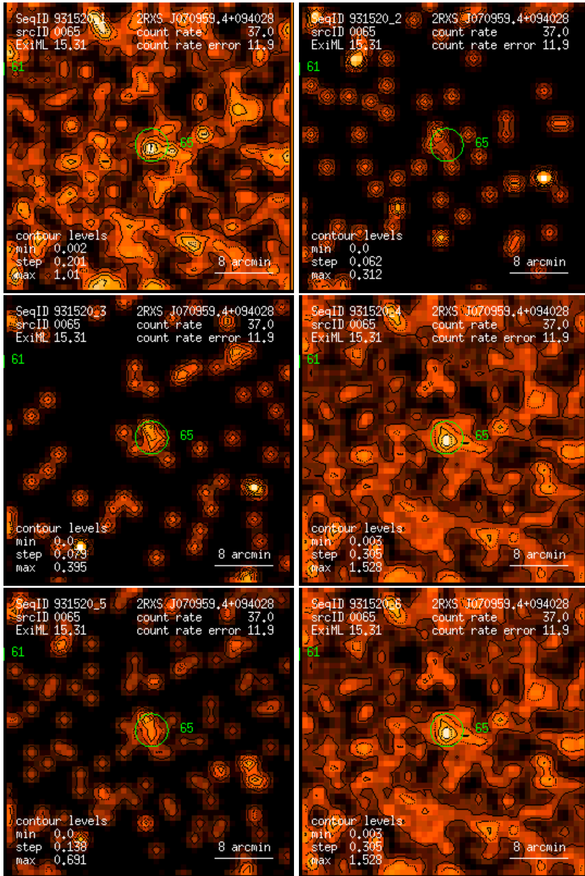
Figure 65: RASS 931520: detection 0065: band rate images, Gaussian filter: (1) PSPC channels 11 – 41, (2) 52 – 90, (3) 91 – 201, (4) 11 – 235, (5) 52 – 201, (6) 11 – 201. Broad band rates in counts/ks. Band rate contour levels in counts/ks/arcmin 2 .
