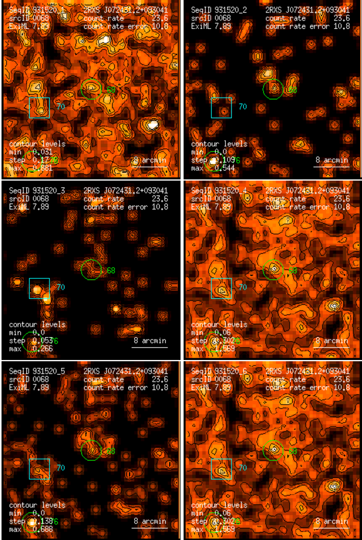
Figure 68: RASS 931520: detection 0068: band rate images, Gaussian filter: (1) PSPC channels 11 – 41, (2) 52 – 90, (3) 91 – 201, (4) 11 – 235, (5) 52 – 201, (6) 11 – 201. Broad band rates in counts/ks. Band rate contour levels in counts/ks/arcmin 2 .
