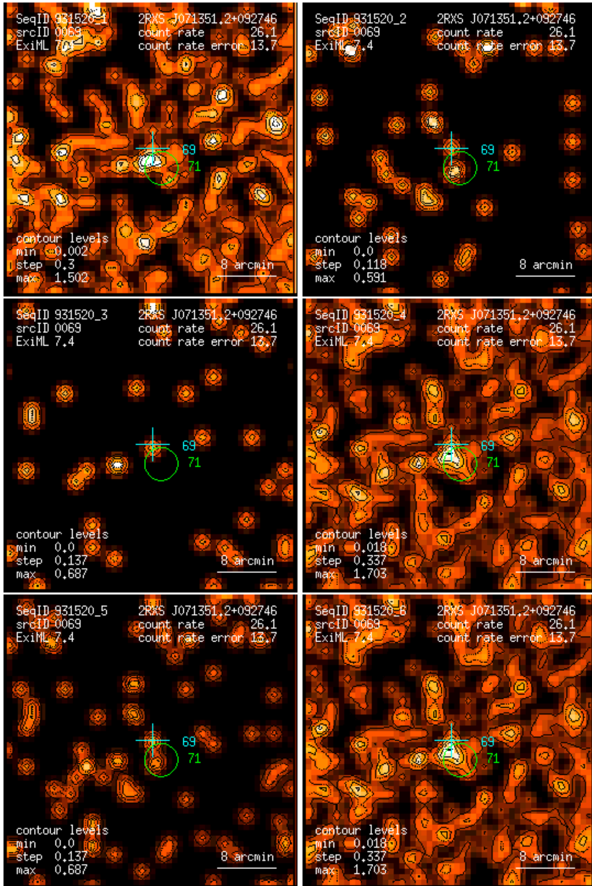
Figure 69: RASS 931520: detection 0069: band rate images, Gaussian filter: (1) PSPC channels 11 – 41, (2) 52 – 90, (3) 91 – 201, (4) 11 – 235, (5) 52 – 201, (6) 11 – 201. Broad band rates in counts/ks. Band rate contour levels in counts/ks/arcmin 2 .
