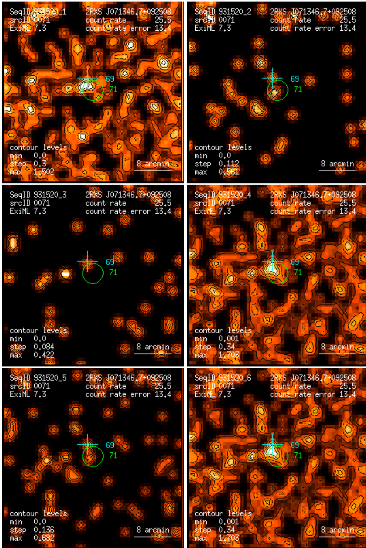
Figure 71: RASS 931520: detection 0071: band rate images, Gaussian filter: (1) PSPC channels 11 – 41, (2) 52 – 90, (3) 91 – 201, (4) 11 – 235, (5) 52 – 201, (6) 11 – 201. Broad band rates in counts/ks. Band rate contour levels in counts/ks/arcmin 2 .
