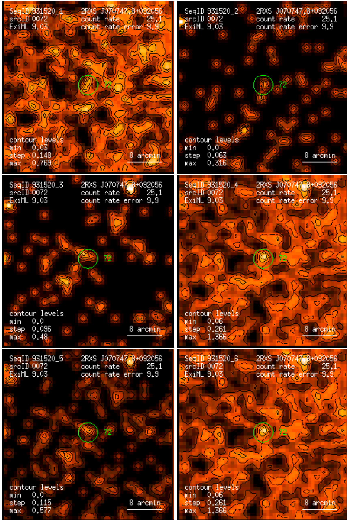
Figure 72: RASS 931520: detection 0072: band rate images, Gaussian filter: (1) PSPC channels 11 – 41, (2) 52 – 90, (3) 91 – 201, (4) 11 – 235, (5) 52 – 201, (6) 11 – 201. Broad band rates in counts/ks. Band rate contour levels in counts/ks/arcmin 2 .
