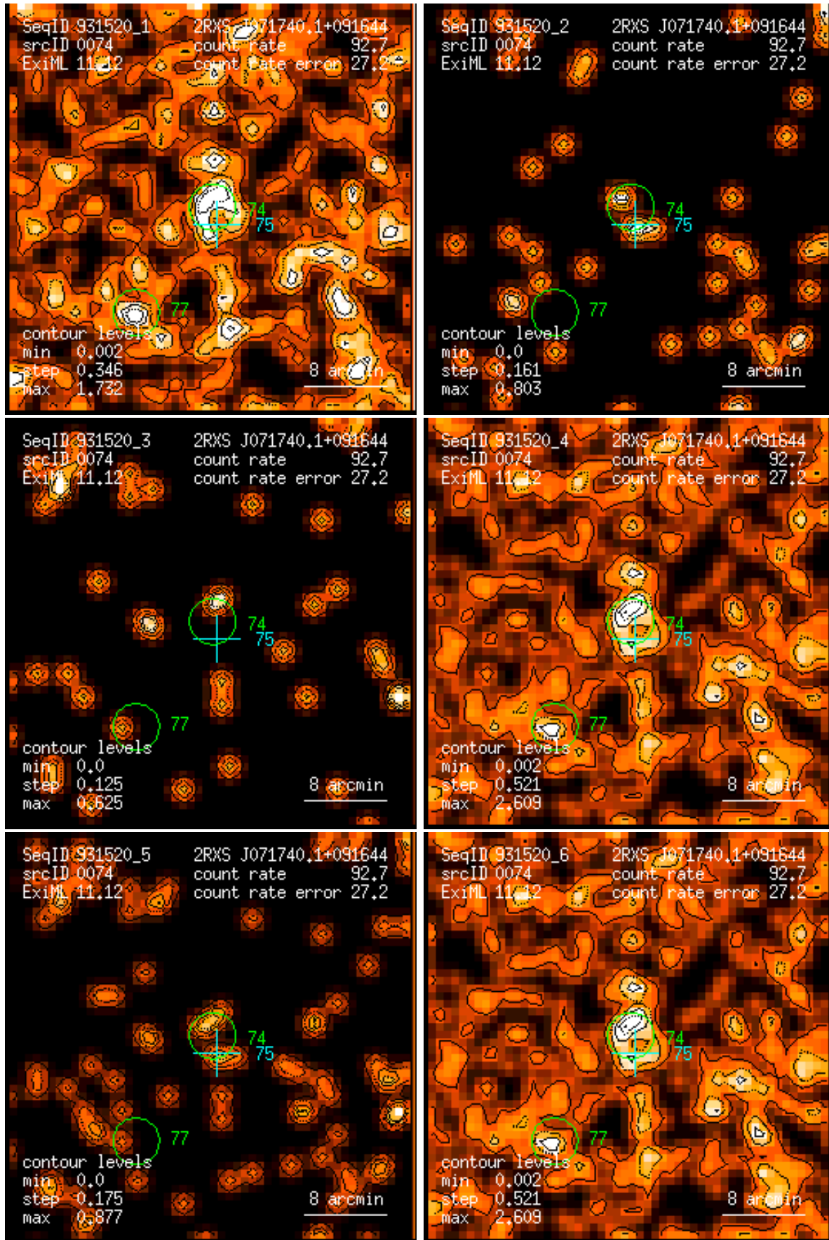
Figure 74: RASS 931520: detection 0074: band rate images, Gaussian filter: (1) PSPC channels 11 – 41, (2) 52 – 90, (3) 91 – 201, (4) 11 – 235, (5) 52 – 201, (6) 11 – 201. Broad band rates in counts/ks. Band rate contour levels in counts/ks/arcmin 2 .
