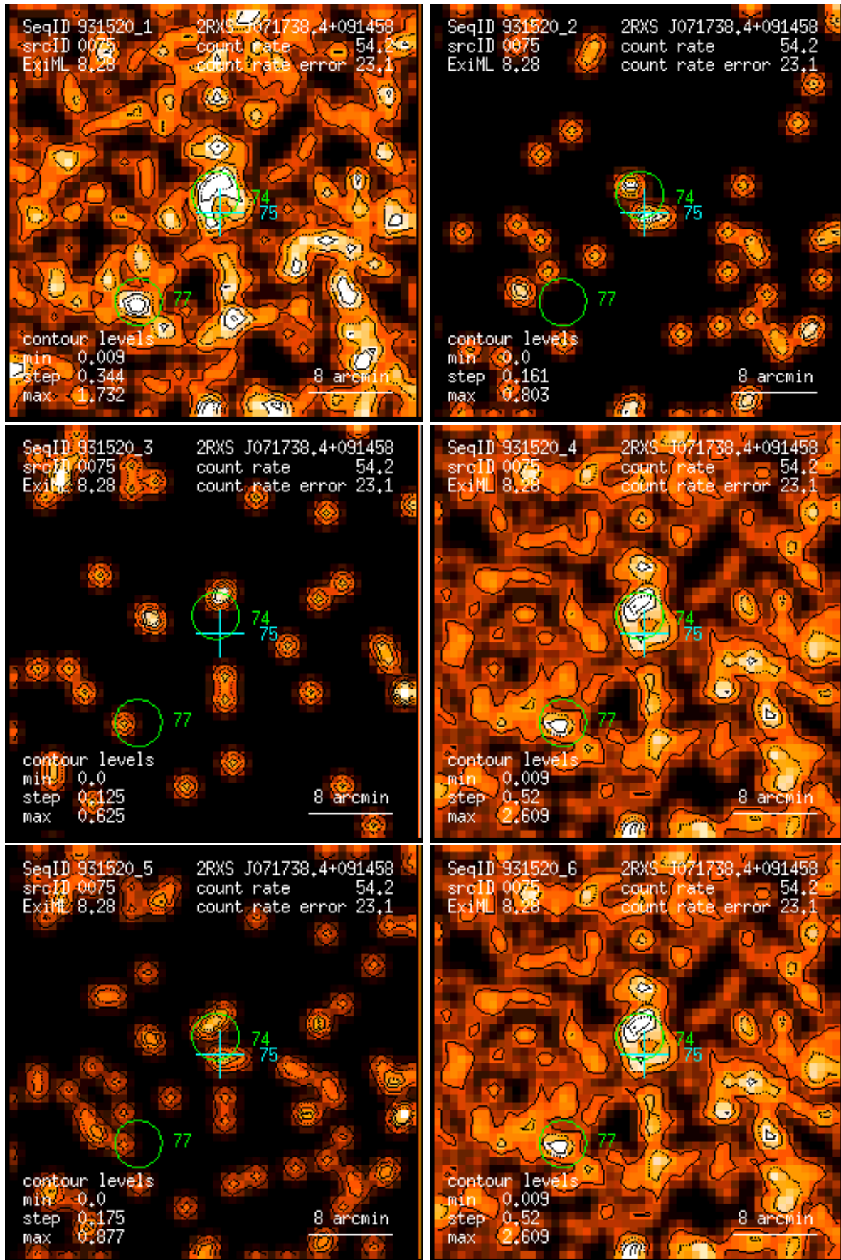
Figure 75: RASS 931520: detection 0075: band rate images, Gaussian filter: (1) PSPC channels 11 – 41, (2) 52 – 90, (3) 91 – 201, (4) 11 – 235, (5) 52 – 201, (6) 11 – 201. Broad band rates in counts/ks. Band rate contour levels in counts/ks/arcmin 2 .
