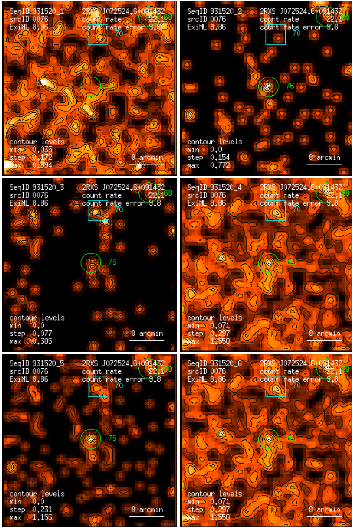
Figure 76: RASS 931520: detection 0076: band rate images, Gaussian filter: (1) PSPC channels 11 – 41, (2) 52 – 90, (3) 91 – 201, (4) 11 – 235, (5) 52 – 201, (6) 11 – 201. Broad band rates in counts/ks. Band rate contour levels in counts/ks/arcmin 2 .
