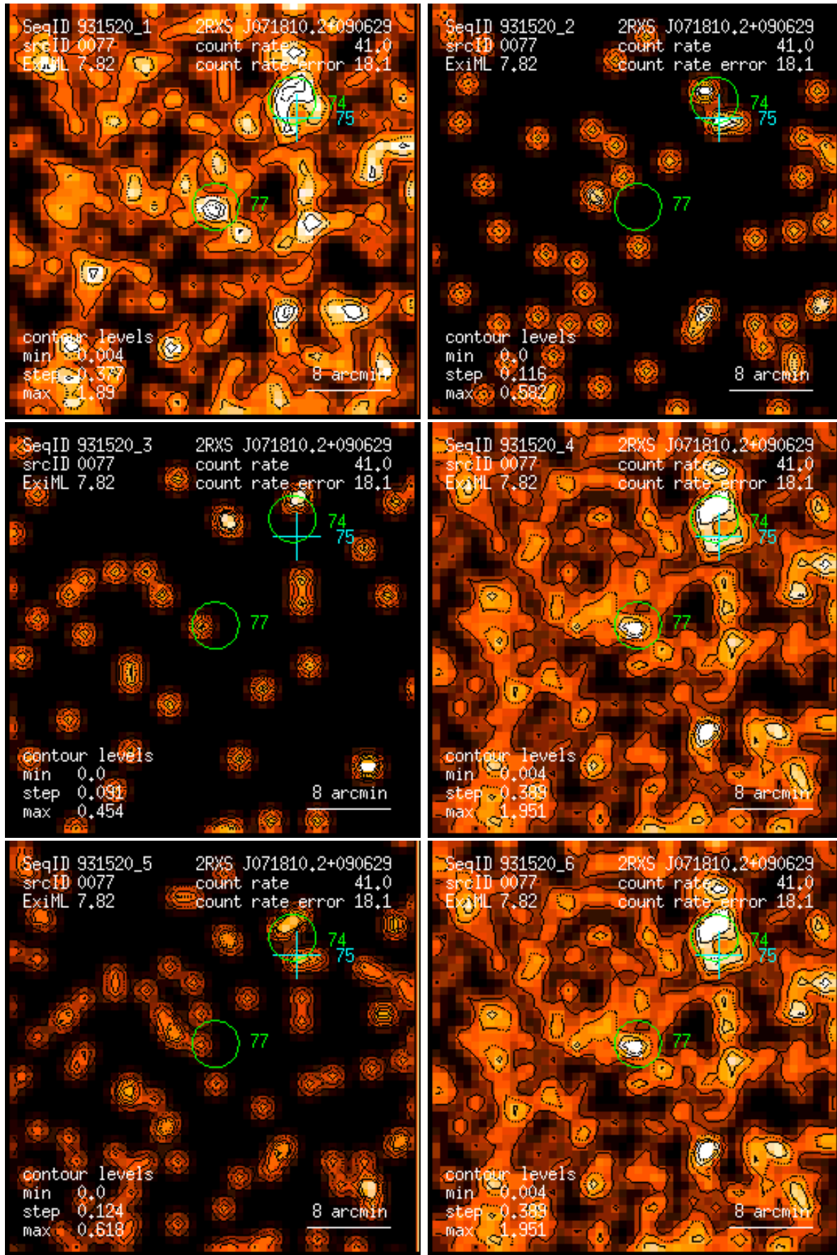
Figure 77: RASS 931520: detection 0077: band rate images, Gaussian filter: (1) PSPC channels 11 – 41, (2) 52 – 90, (3) 91 – 201, (4) 11 – 235, (5) 52 – 201, (6) 11 – 201. Broad band rates in counts/ks. Band rate contour levels in counts/ks/arcmin 2 .
