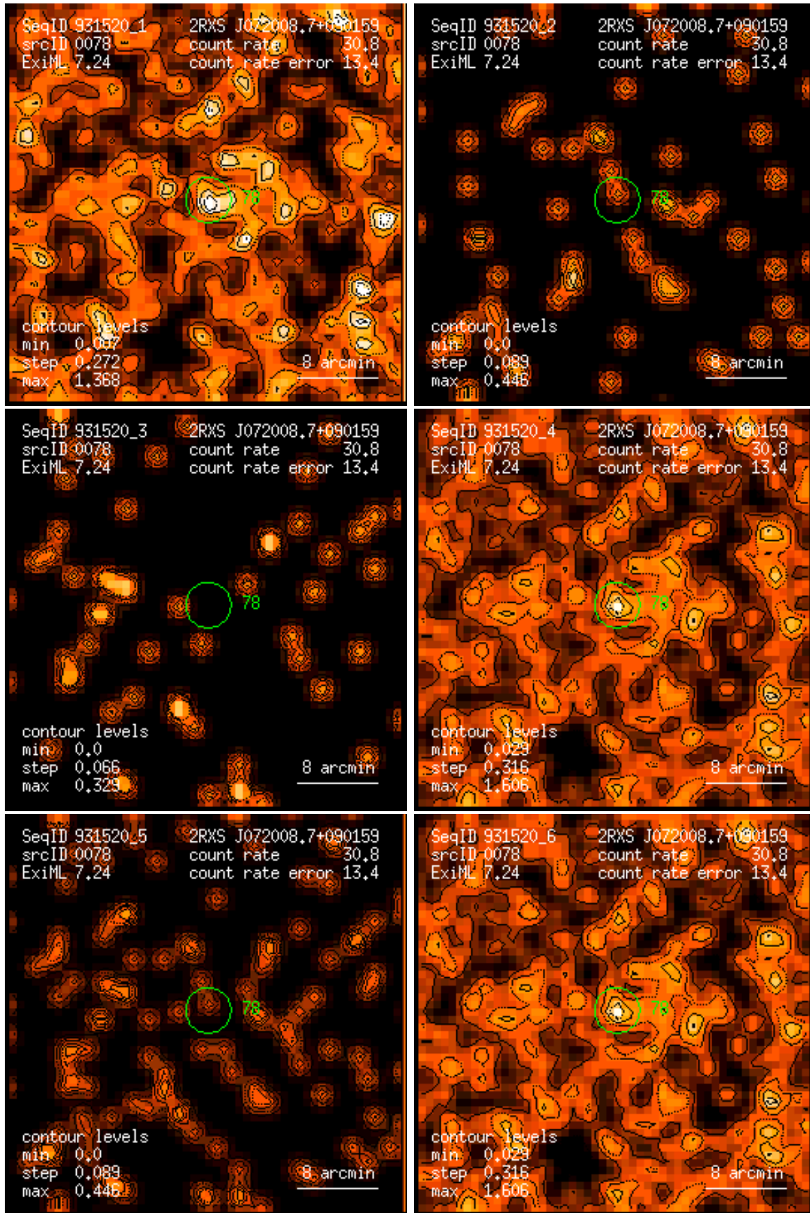
Figure 78: RASS 931520: detection 0078: band rate images, Gaussian filter: (1) PSPC channels 11 – 41, (2) 52 – 90, (3) 91 – 201, (4) 11 – 235, (5) 52 – 201, (6) 11 – 201. Broad band rates in counts/ks. Band rate contour levels in counts/ks/arcmin 2 .
