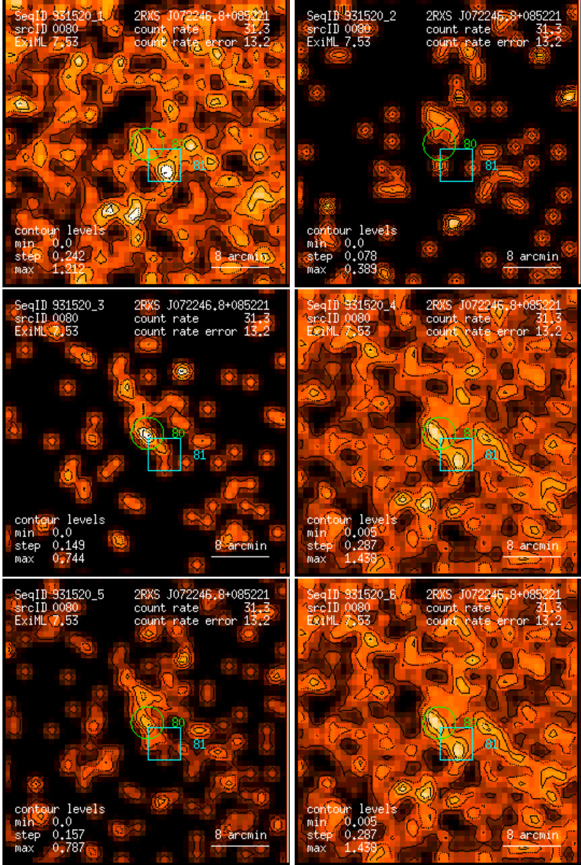
Figure 80: RASS 931520: detection 0080: band rate images, Gaussian filter: (1) PSPC channels 11 – 41, (2) 52 – 90, (3) 91 – 201, (4) 11 – 235, (5) 52 – 201, (6) 11 – 201. Broad band rates in counts/ks. Band rate contour levels in counts/ks/arcmin 2 .
