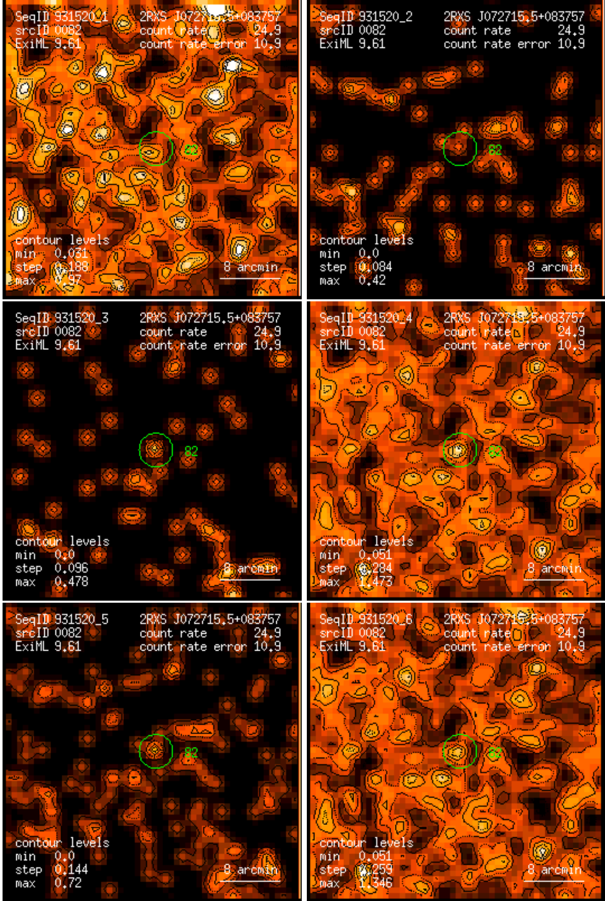
Figure 82: RASS 931520: detection 0082: band rate images, Gaussian filter: (1) PSPC channels 11 – 41, (2) 52 – 90, (3) 91 – 201, (4) 11 – 235, (5) 52 – 201, (6) 11 – 201. Broad band rates in counts/ks. Band rate contour levels in counts/ks/arcmin 2 .
