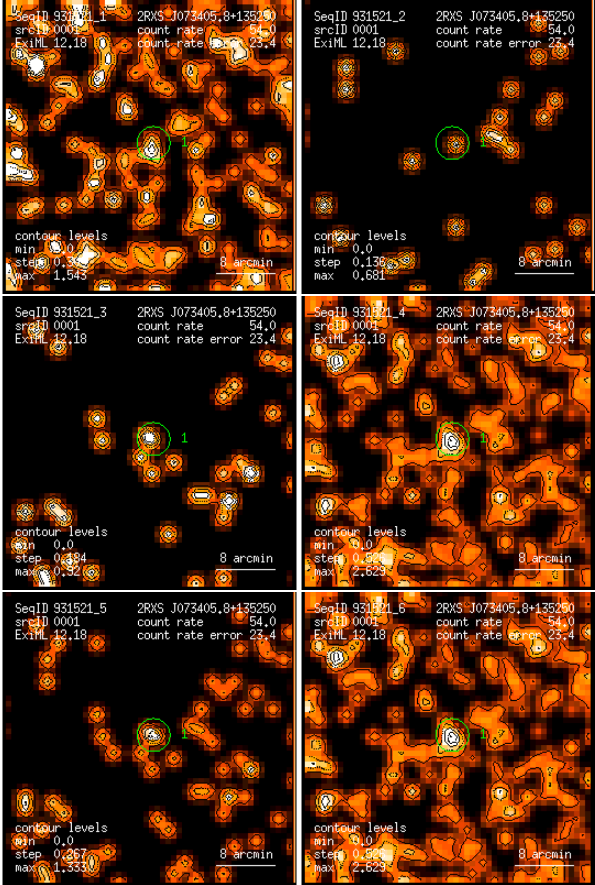
Figure 1: RASS 931521: detection 0001: band rate images, Gaussian filter: (1) PSPC channels 11 – 41, (2) 52 – 90, (3) 91 – 201, (4) 11 – 235, (5) 52 – 201, (6) 11 – 201. Broad band rates in counts/ks. Band rate contour levels in counts/ks/arcmin 2 .
