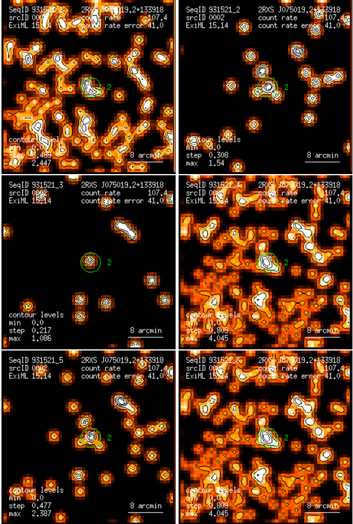
Figure 2: RASS 931521: detection 0002: band rate images, Gaussian filter: (1) PSPC channels 11 – 41, (2) 52 – 90, (3) 91 – 201, (4) 11 – 235, (5) 52 – 201, (6) 11 – 201. Broad band rates in counts/ks. Band rate contour levels in counts/ks/arcmin 2 .
