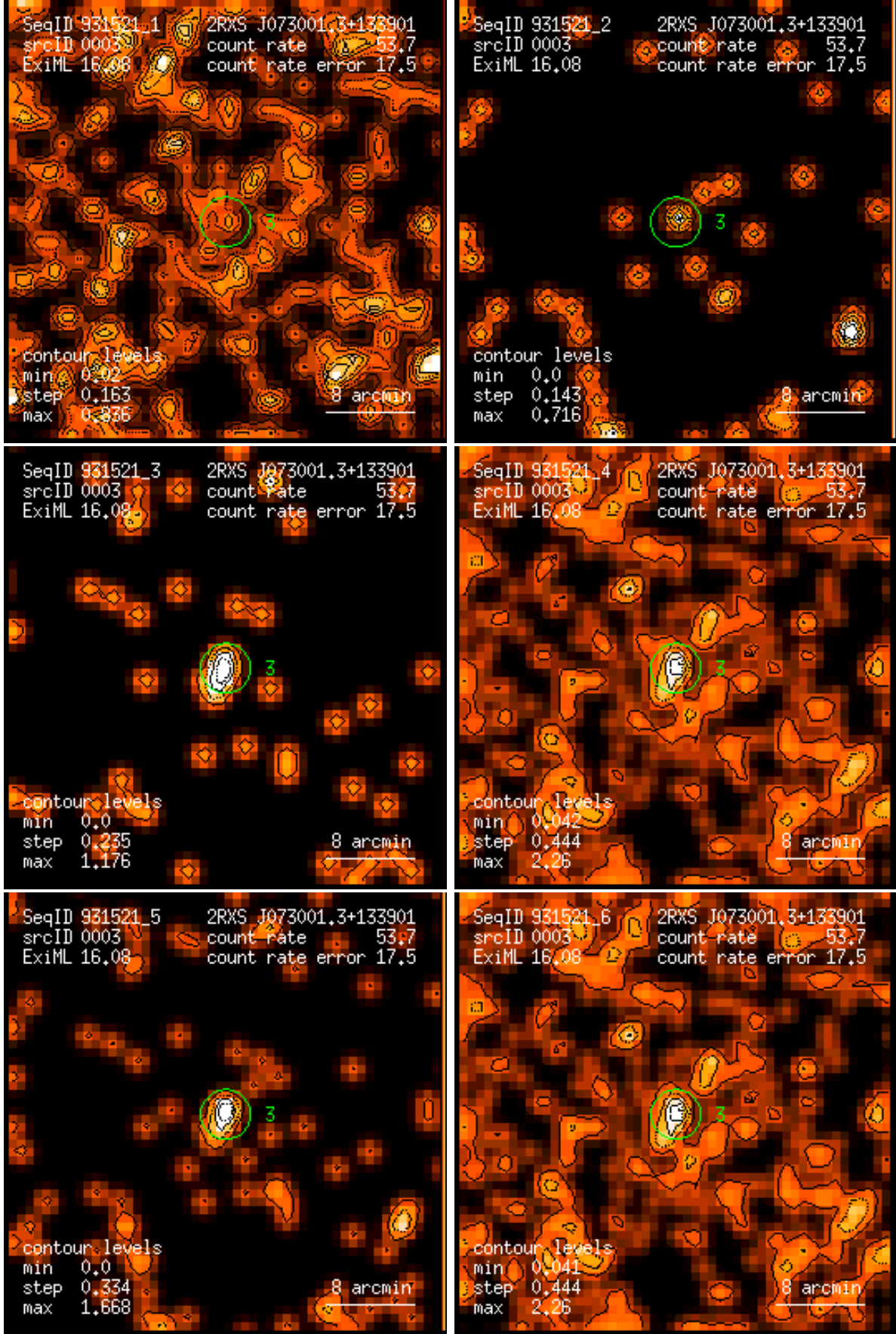
Figure 3: RASS 931521: detection 0003: band rate images, Gaussian filter: (1) PSPC channels 11 – 41, (2) 52 – 90, (3) 91 – 201, (4) 11 – 235, (5) 52 – 201, (6) 11 – 201. Broad band rates in counts/ks. Band rate contour levels in counts/ks/arcmin 2 .
