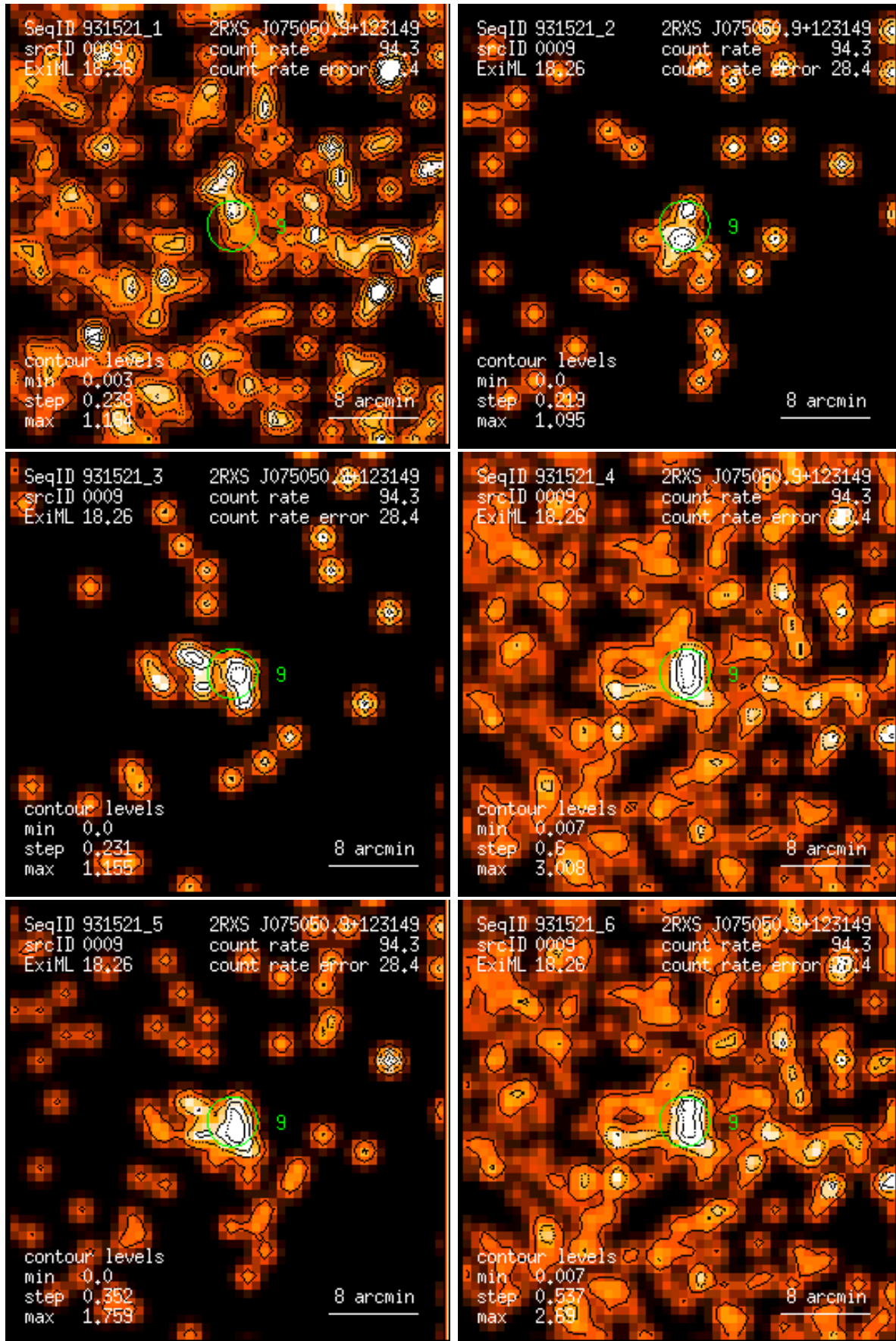
Figure 9: RASS 931521: detection 0009: band rate images, Gaussian filter: (1) PSPC channels 11 – 41, (2) 52 – 90, (3) 91 – 201, (4) 11 – 235, (5) 52 – 201, (6) 11 – 201. Broad band rates in counts/ks. Band rate contour levels in counts/ks/arcmin 2 .
