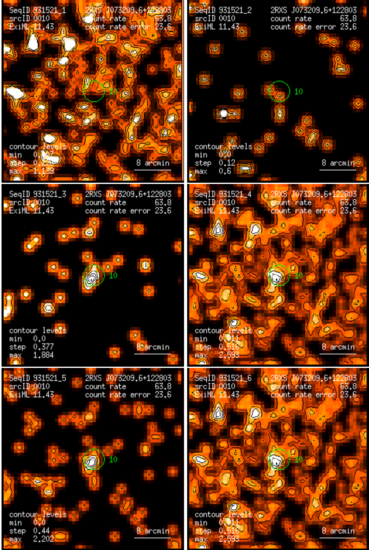
Figure 10: RASS 931521: detection 0010: band rate images, Gaussian filter: (1) PSPC channels 11 – 41, (2) 52 – 90, (3) 91 – 201, (4) 11 – 235, (5) 52 – 201, (6) 11 – 201. Broad band rates in counts/ks. Band rate contour levels in counts/ks/arcmin 2 .
