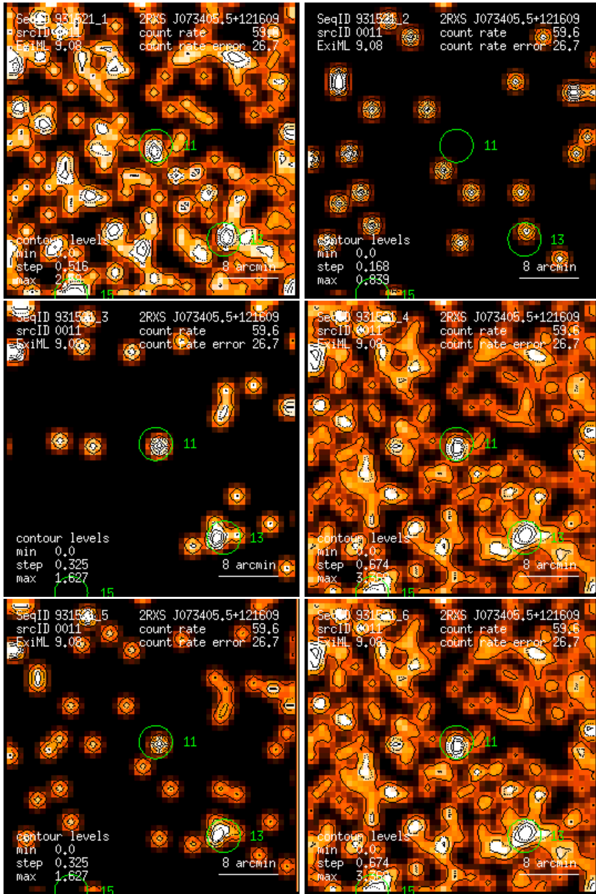
Figure 11: RASS 931521: detection 0011: band rate images, Gaussian filter: (1) PSPC channels 11 – 41, (2) 52 – 90, (3) 91 – 201, (4) 11 – 235, (5) 52 – 201, (6) 11 – 201. Broad band rates in counts/ks. Band rate contour levels in counts/ks/arcmin 2 .
