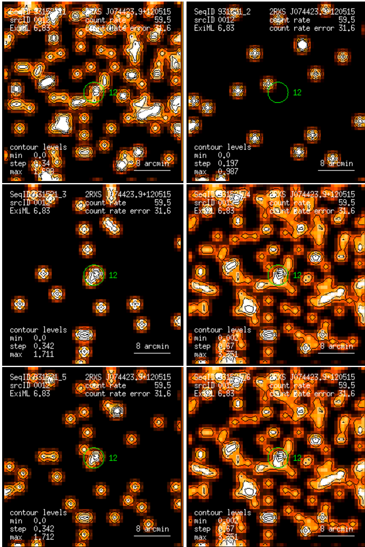
Figure 12: RASS 931521: detection 0012: band rate images, Gaussian filter: (1) PSPC channels 11 – 41, (2) 52 – 90, (3) 91 – 201, (4) 11 – 235, (5) 52 – 201, (6) 11 – 201. Broad band rates in counts/ks. Band rate contour levels in counts/ks/arcmin 2 .
