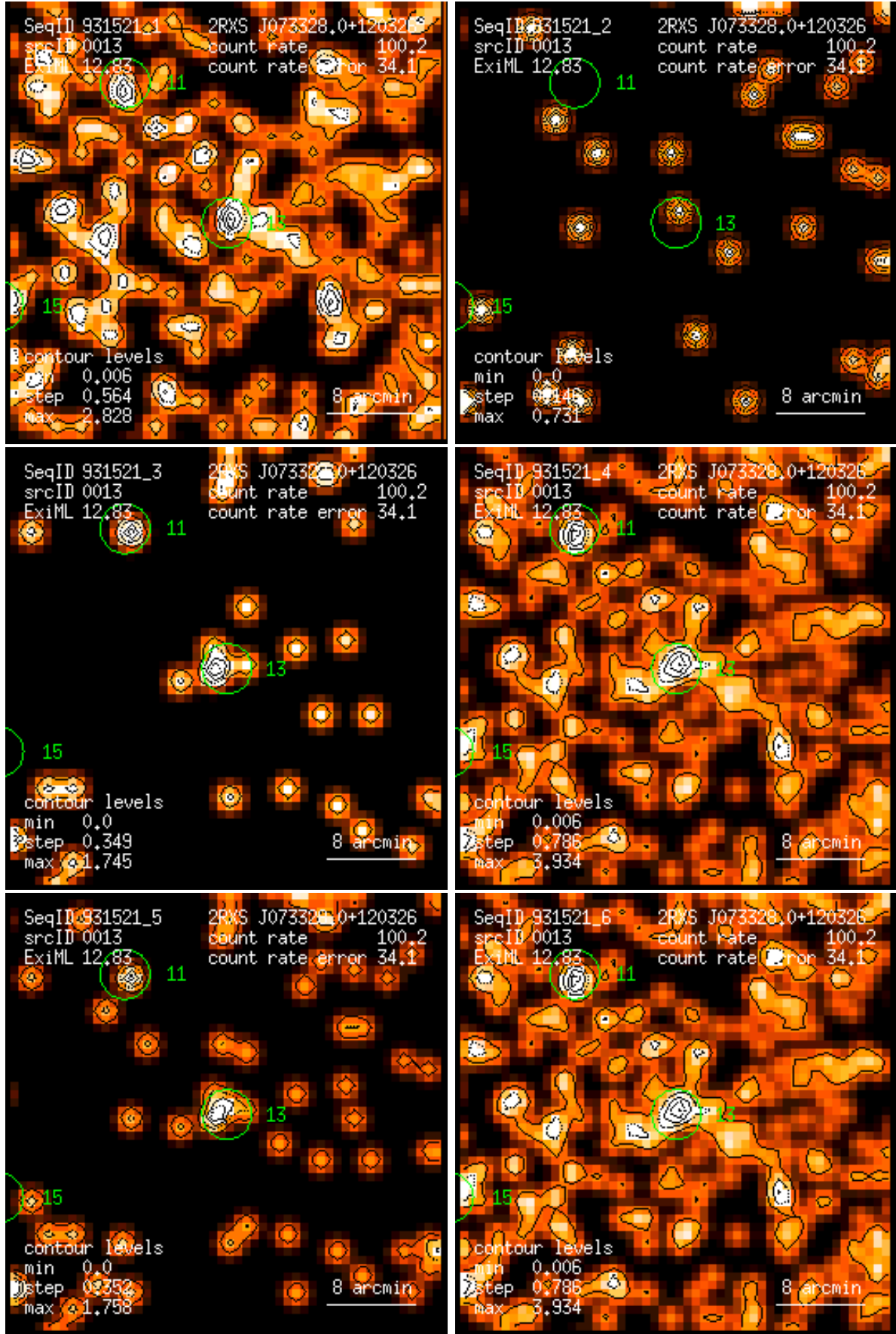
Figure 13: RASS 931521: detection 0013: band rate images, Gaussian filter: (1) PSPC channels 11 – 41, (2) 52 – 90, (3) 91 – 201, (4) 11 – 235, (5) 52 – 201, (6) 11 – 201. Broad band rates in counts/ks. Band rate contour levels in counts/ks/arcmin 2 .
