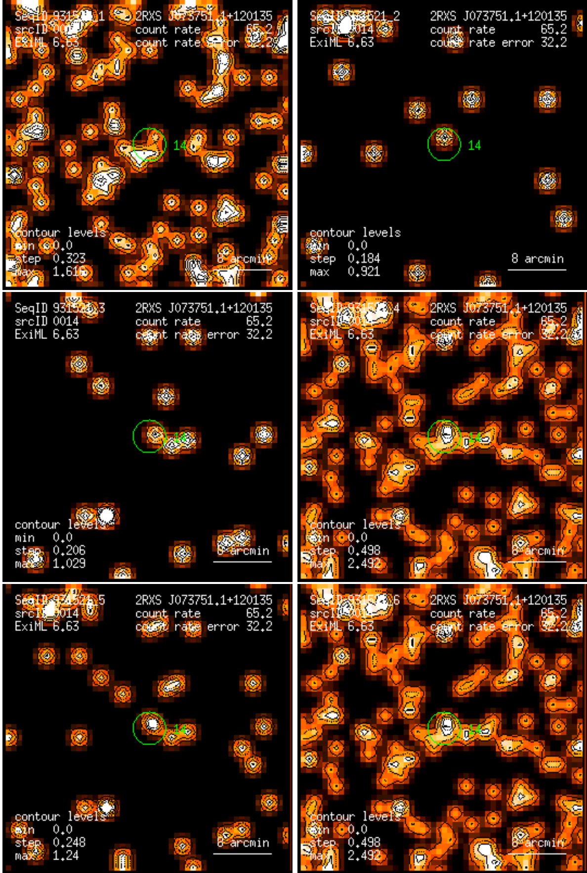
Figure 14: RASS 931521: detection 0014: band rate images, Gaussian filter: (1) PSPC channels 11 – 41, (2) 52 – 90, (3) 91 – 201, (4) 11 – 235, (5) 52 – 201, (6) 11 – 201. Broad band rates in counts/ks. Band rate contour levels in counts/ks/arcmin 2 .
