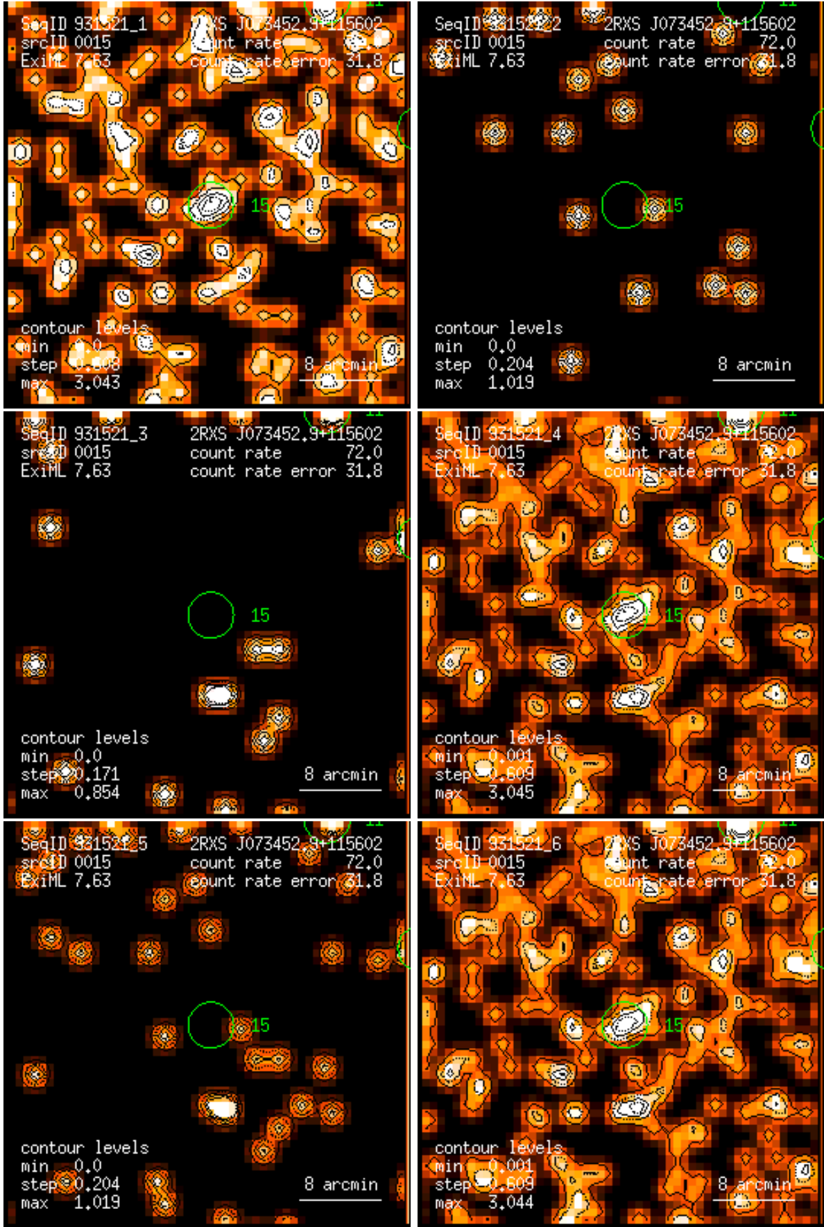
Figure 15: RASS 931521: detection 0015: band rate images, Gaussian filter: (1) PSPC channels 11 – 41, (2) 52 – 90, (3) 91 – 201, (4) 11 – 235, (5) 52 – 201, (6) 11 – 201. Broad band rates in counts/ks. Band rate contour levels in counts/ks/arcmin 2 .
