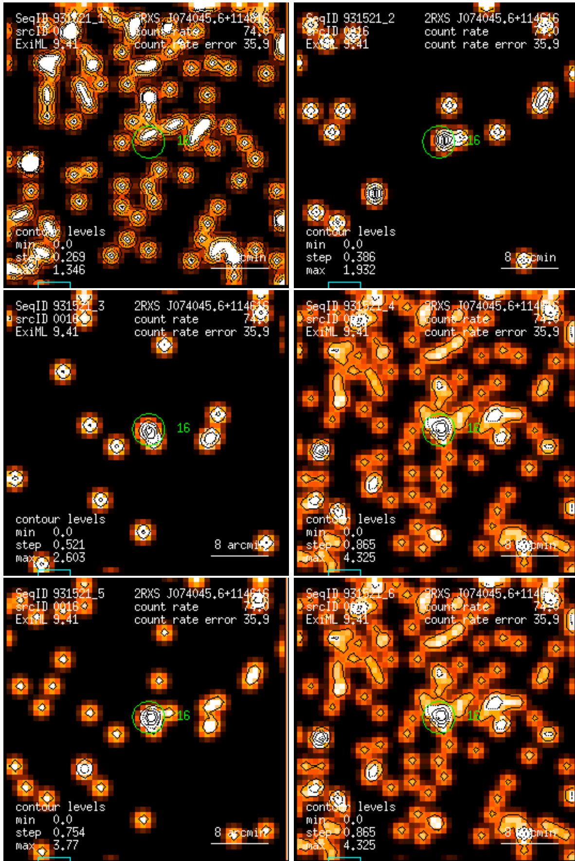
Figure 16: RASS 931521: detection 0016: band rate images, Gaussian filter: (1) PSPC channels 11 – 41, (2) 52 – 90, (3) 91 – 201, (4) 11 – 235, (5) 52 – 201, (6) 11 – 201. Broad band rates in counts/ks. Band rate contour levels in counts/ks/arcmin 2 .
