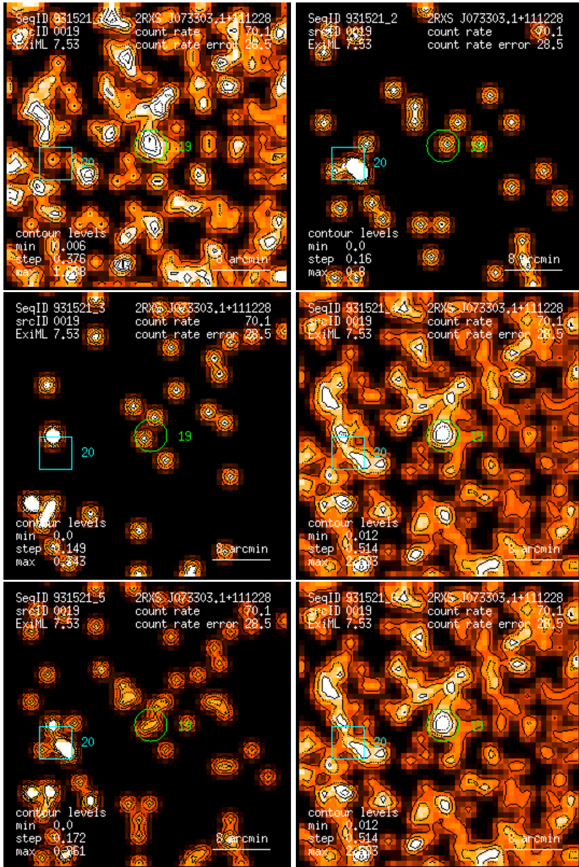
Figure 19: RASS 931521: detection 0019: band rate images, Gaussian filter: (1) PSPC channels 11 – 41, (2) 52 – 90, (3) 91 – 201, (4) 11 – 235, (5) 52 – 201, (6) 11 – 201. Broad band rates in counts/ks. Band rate contour levels in counts/ks/arcmin 2 .
