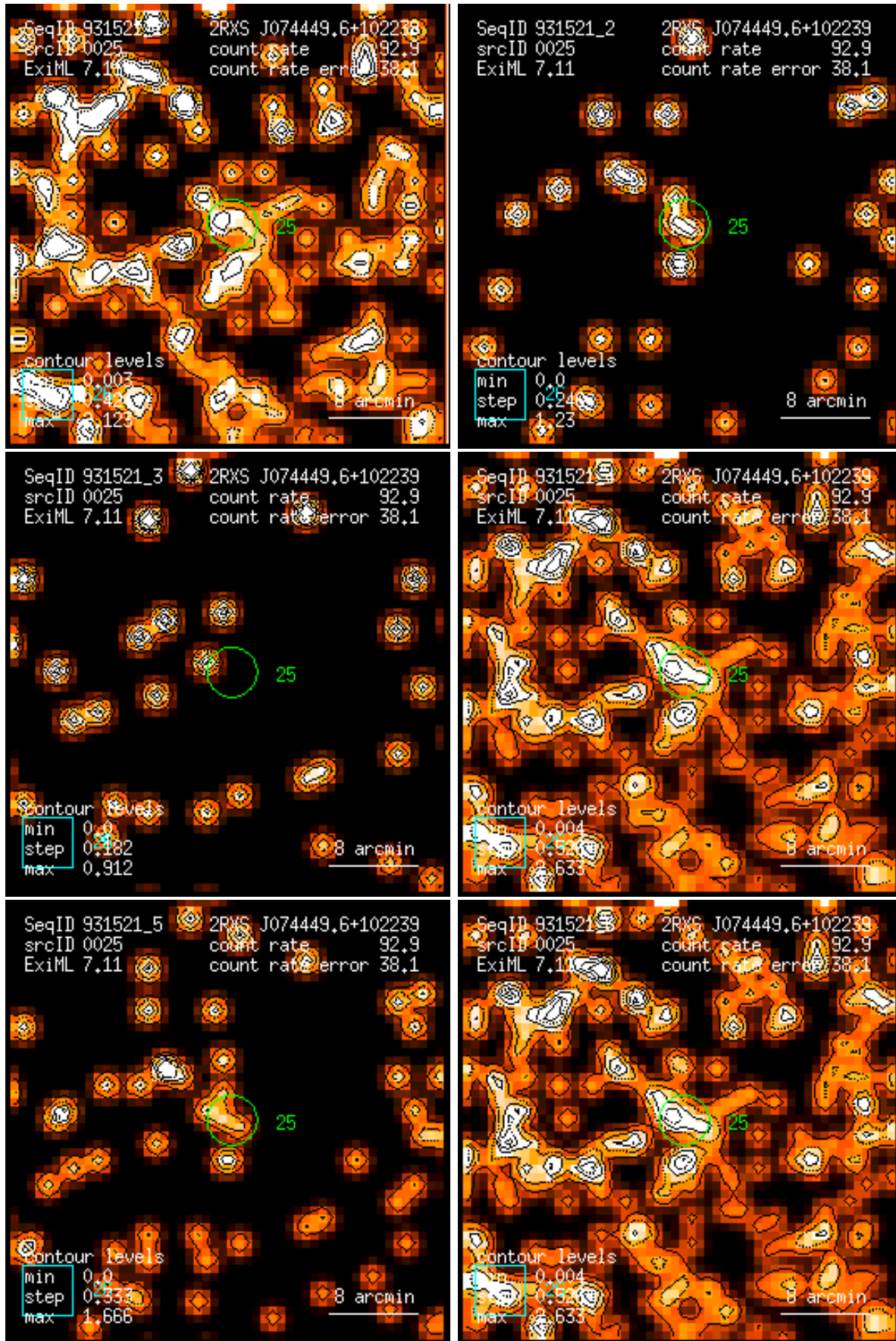
Figure 25: RASS 931521: detection 0025: band rate images, Gaussian filter: (1) PSPC channels 11 – 41, (2) 52 – 90, (3) 91 – 201, (4) 11 – 235, (5) 52 – 201, (6) 11 – 201. Broad band rates in counts/ks. Band rate contour levels in counts/ks/arcmin 2 .
