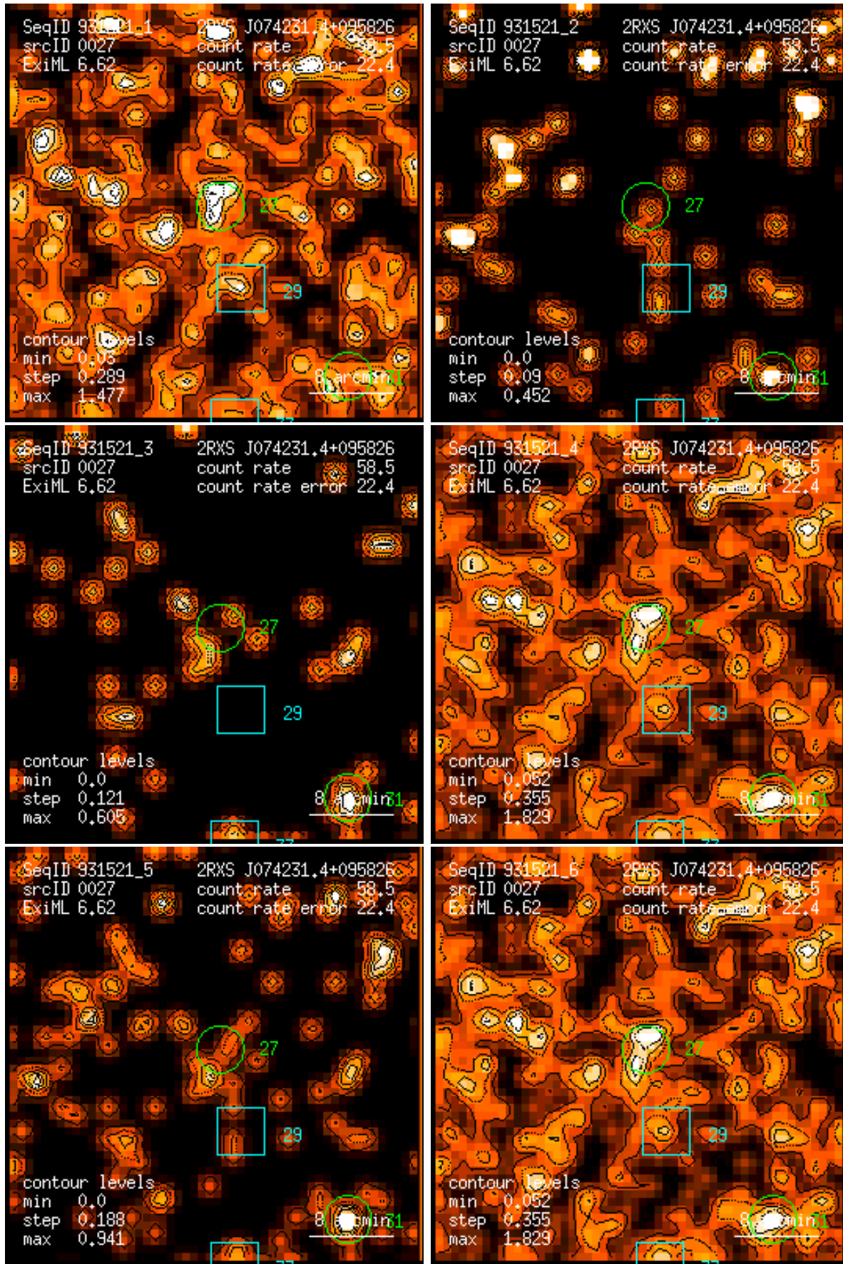
Figure 27: RASS 931521: detection 0027: band rate images, Gaussian filter: (1) PSPC channels 11 – 41, (2) 52 – 90, (3) 91 – 201, (4) 11 – 235, (5) 52 – 201, (6) 11 – 201. Broad band rates in counts/ks. Band rate contour levels in counts/ks/arcmin 2 .
