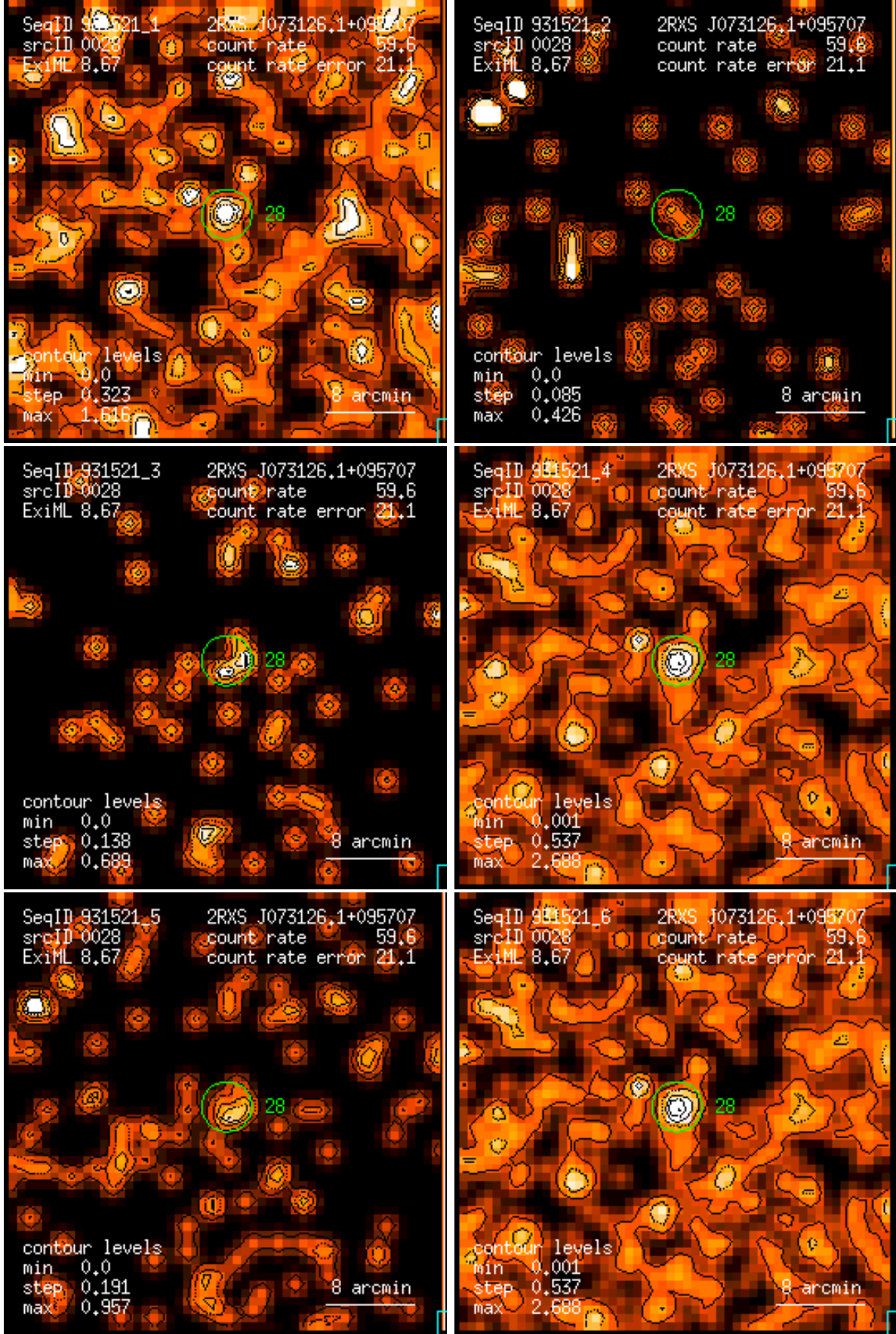
Figure 28: RASS 931521: detection 0028: band rate images, Gaussian filter: (1) PSPC channels 11 – 41, (2) 52 – 90, (3) 91 – 201, (4) 11 – 235, (5) 52 – 201, (6) 11 – 201. Broad band rates in counts/ks. Band rate contour levels in counts/ks/arcmin 2 .
