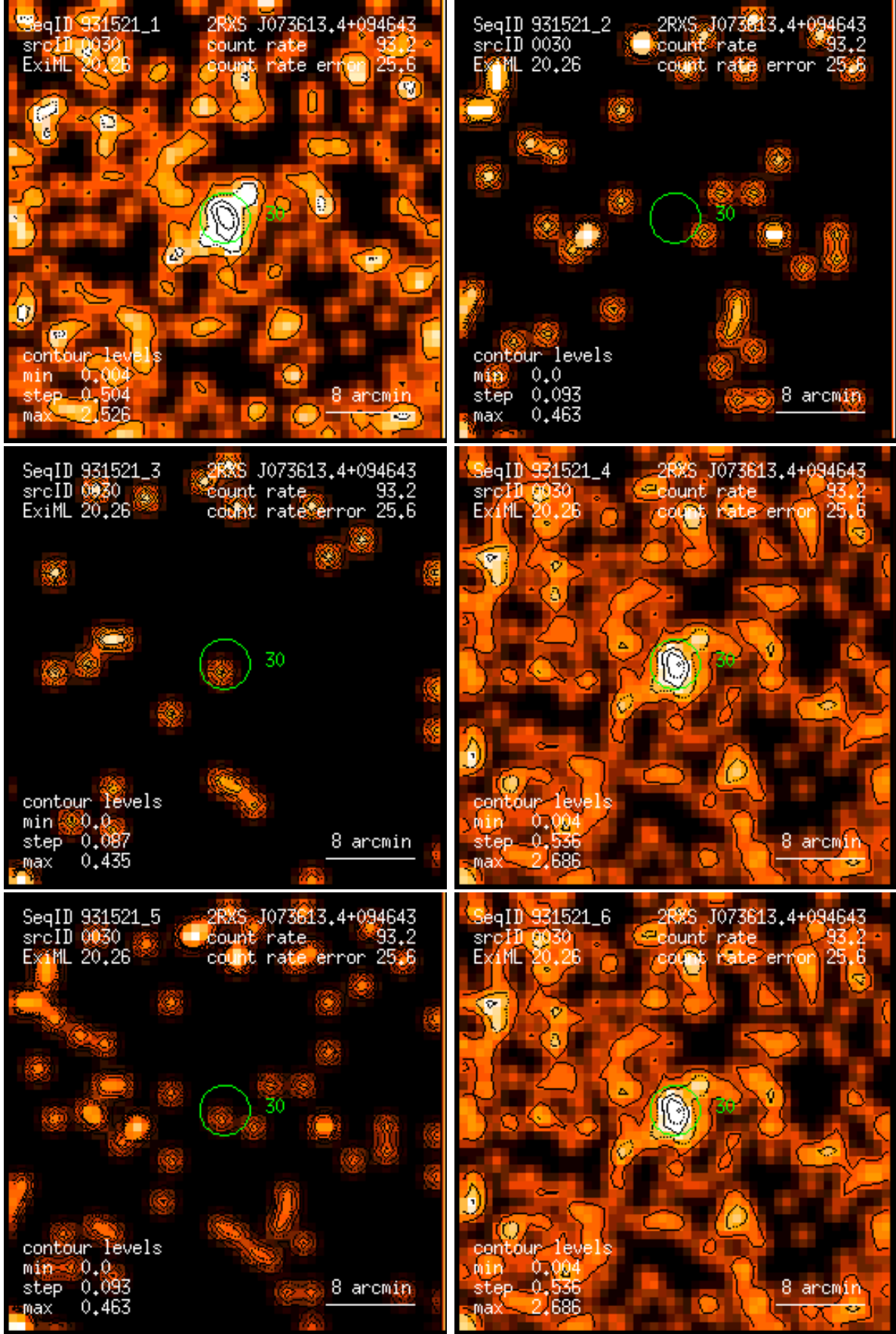
Figure 30: RASS 931521: detection 0030: band rate images, Gaussian filter: (1) PSPC channels 11 – 41, (2) 52 – 90, (3) 91 – 201, (4) 11 – 235, (5) 52 – 201, (6) 11 – 201. Broad band rates in counts/ks. Band rate contour levels in counts/ks/arcmin 2 .
