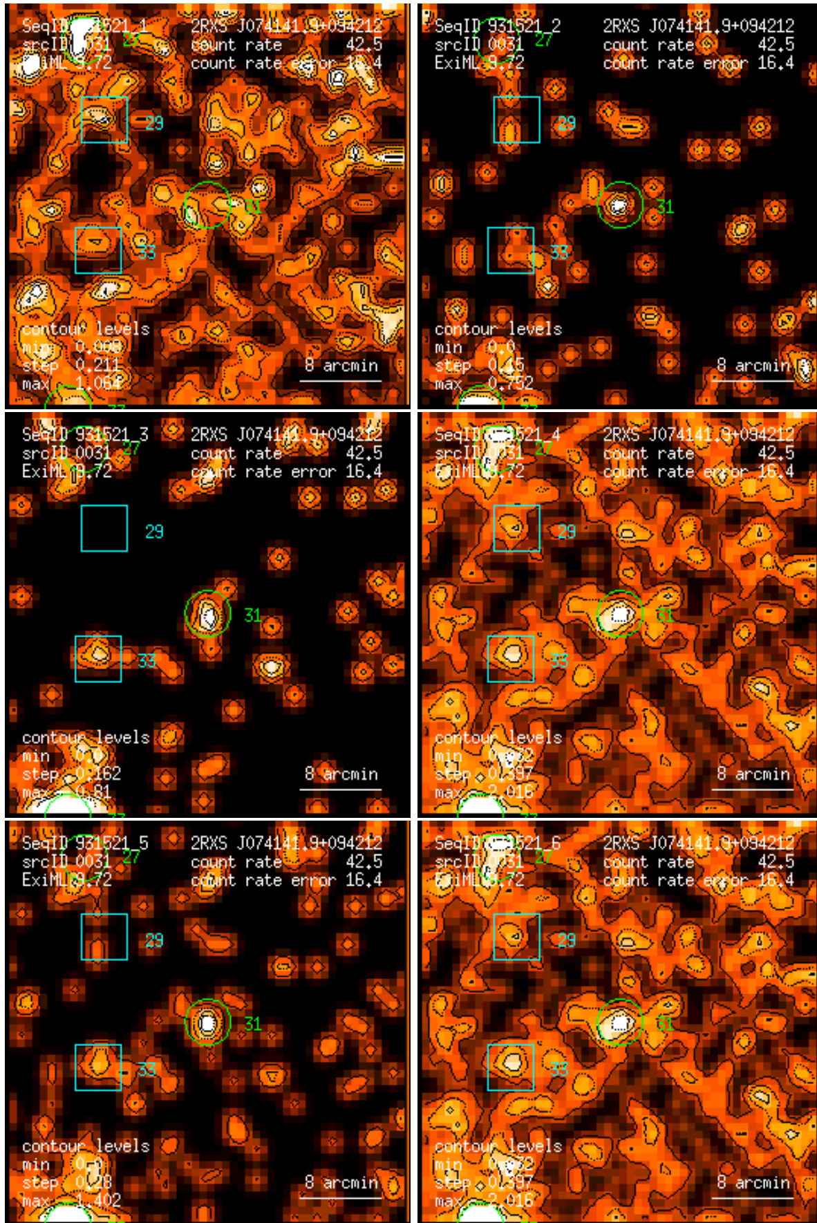
Figure 31: RASS 931521: detection 0031: band rate images, Gaussian filter: (1) PSPC channels 11 – 41, (2) 52 – 90, (3) 91 – 201, (4) 11 – 235, (5) 52 – 201, (6) 11 – 201. Broad band rates in counts/ks. Band rate contour levels in counts/ks/arcmin 2 .
