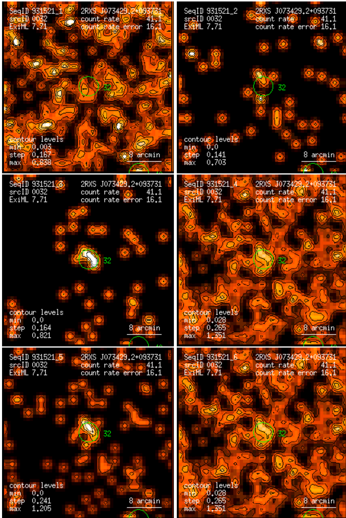
Figure 32: RASS 931521: detection 0032: band rate images, Gaussian filter: (1) PSPC channels 11 – 41, (2) 52 – 90, (3) 91 – 201, (4) 11 – 235, (5) 52 – 201, (6) 11 – 201. Broad band rates in counts/ks. Band rate contour levels in counts/ks/arcmin 2 .
