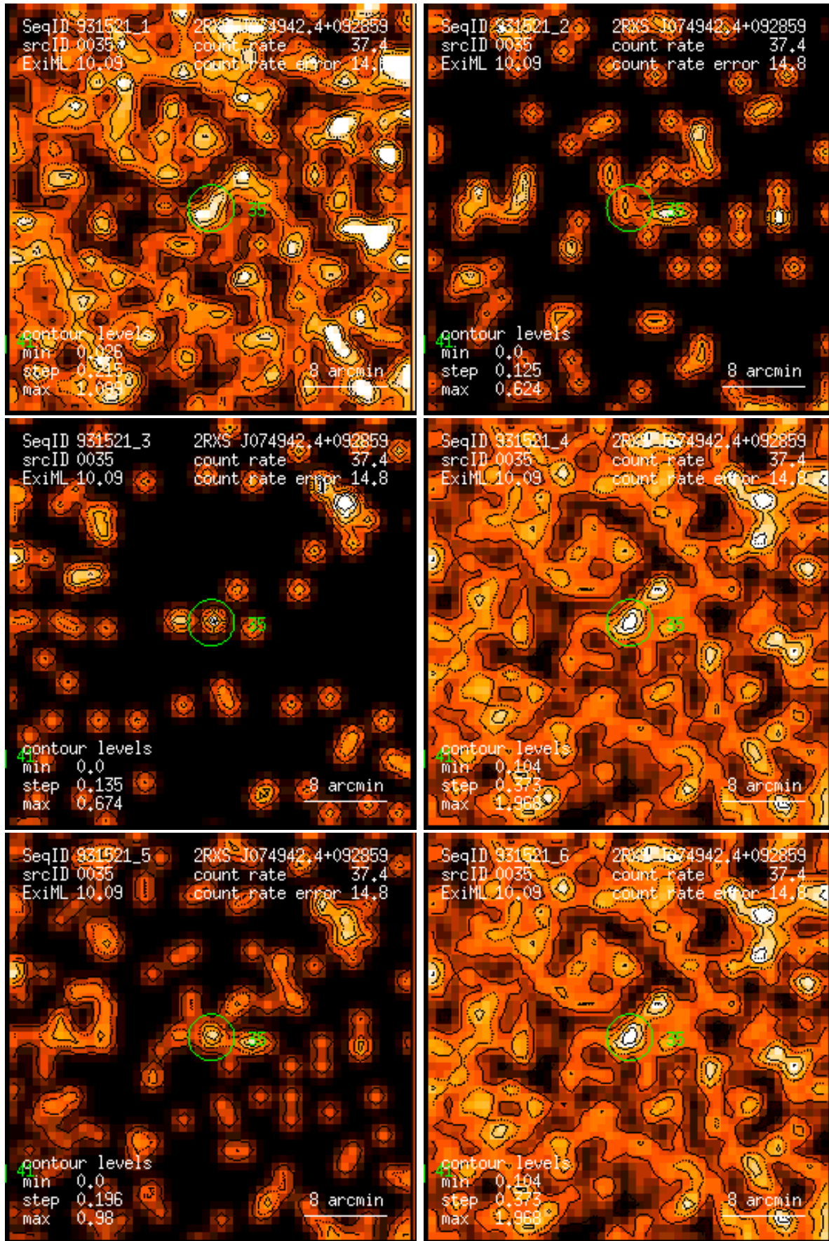
Figure 35: RASS 931521: detection 0035: band rate images, Gaussian filter: (1) PSPC channels 11 – 41, (2) 52 – 90, (3) 91 – 201, (4) 11 – 235, (5) 52 – 201, (6) 11 – 201. Broad band rates in counts/ks. Band rate contour levels in counts/ks/arcmin 2 .
