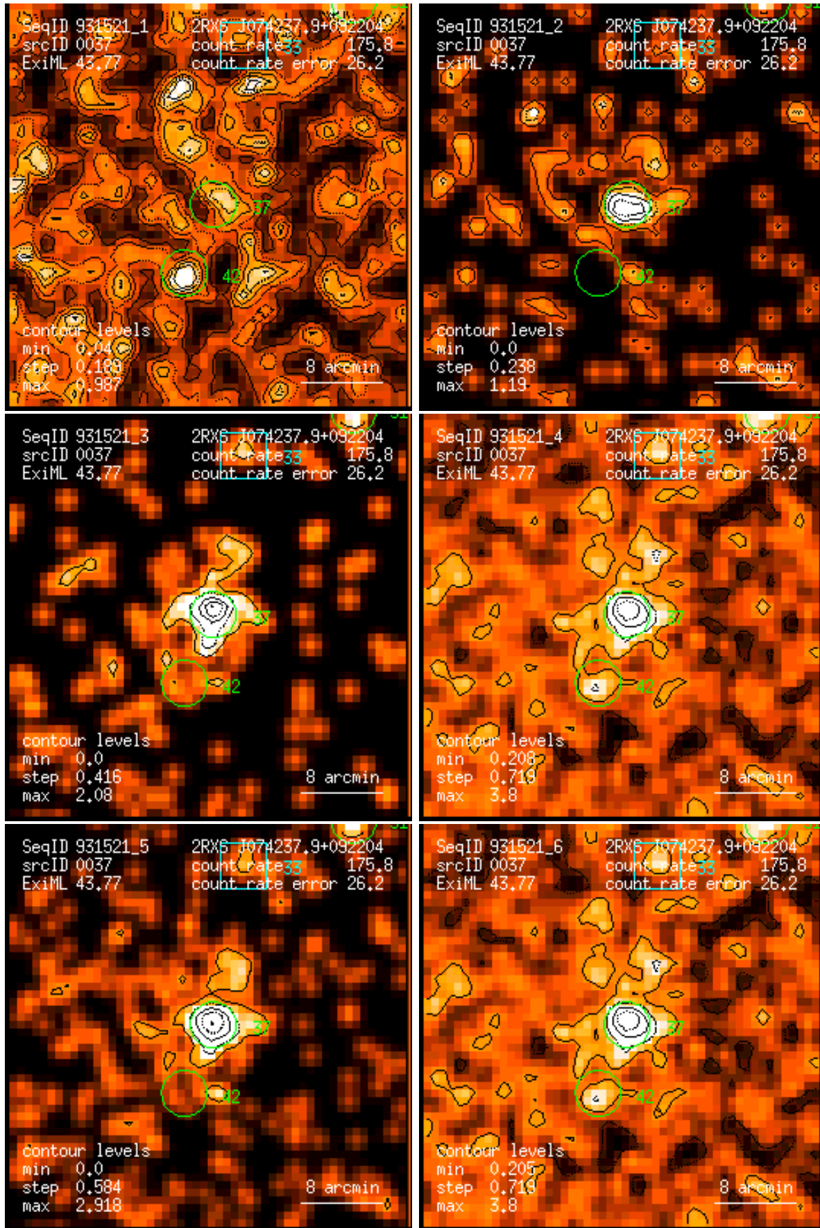
Figure 37: RASS 931521: detection 0037: band rate images, Gaussian filter: (1) PSPC channels 11 – 41, (2) 52 – 90, (3) 91 – 201, (4) 11 – 235, (5) 52 – 201, (6) 11 – 201. Broad band rates in counts/ks. Band rate contour levels in counts/ks/arcmin 2 .
