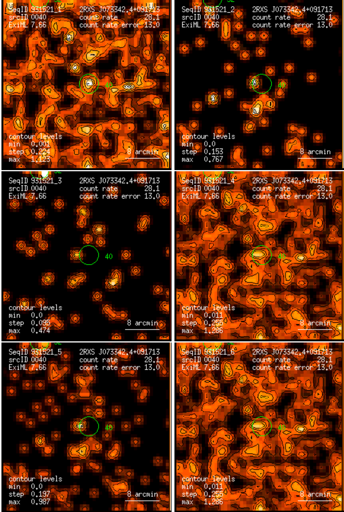
Figure 40: RASS 931521: detection 0040: band rate images, Gaussian filter: (1) PSPC channels 11 – 41, (2) 52 – 90, (3) 91 – 201, (4) 11 – 235, (5) 52 – 201, (6) 11 – 201. Broad band rates in counts/ks. Band rate contour levels in counts/ks/arcmin 2 .
