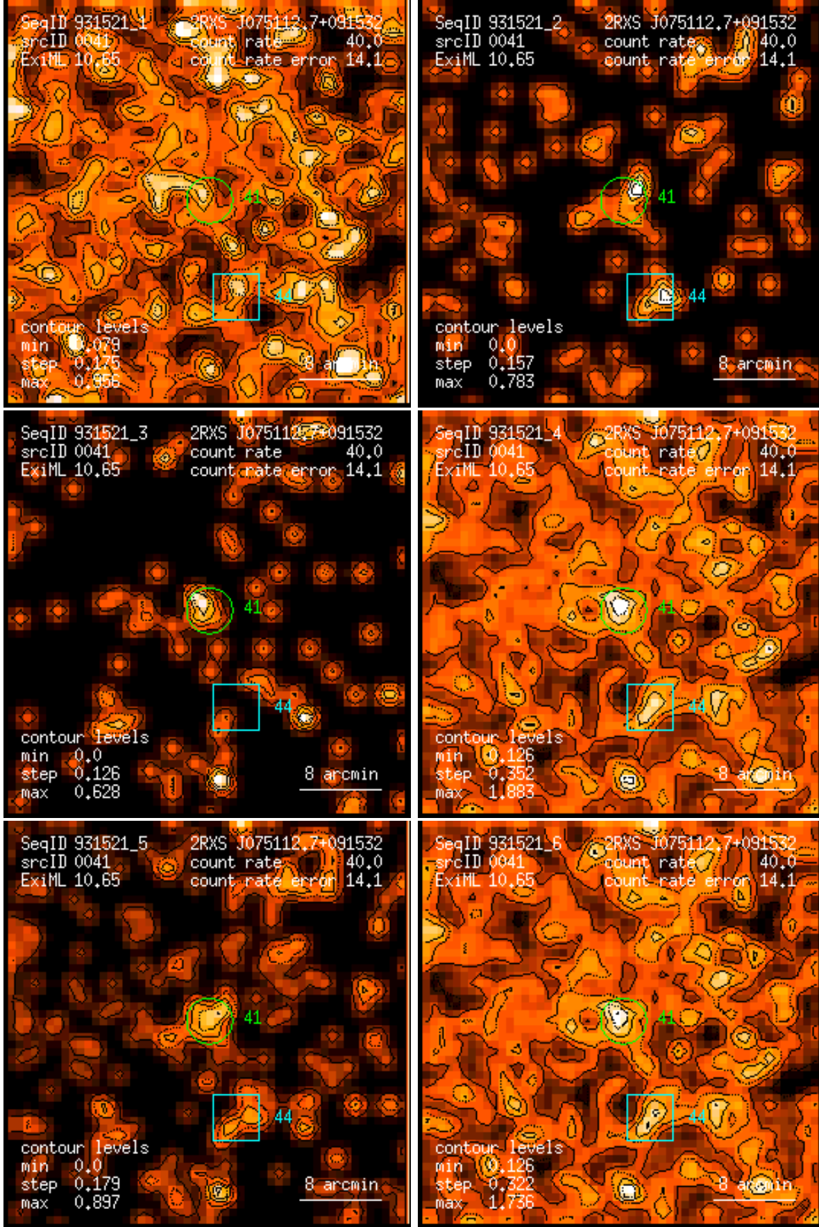
Figure 41: RASS 931521: detection 0041: band rate images, Gaussian filter: (1) PSPC channels 11 – 41, (2) 52 – 90, (3) 91 – 201, (4) 11 – 235, (5) 52 – 201, (6) 11 – 201. Broad band rates in counts/ks. Band rate contour levels in counts/ks/arcmin 2 .
