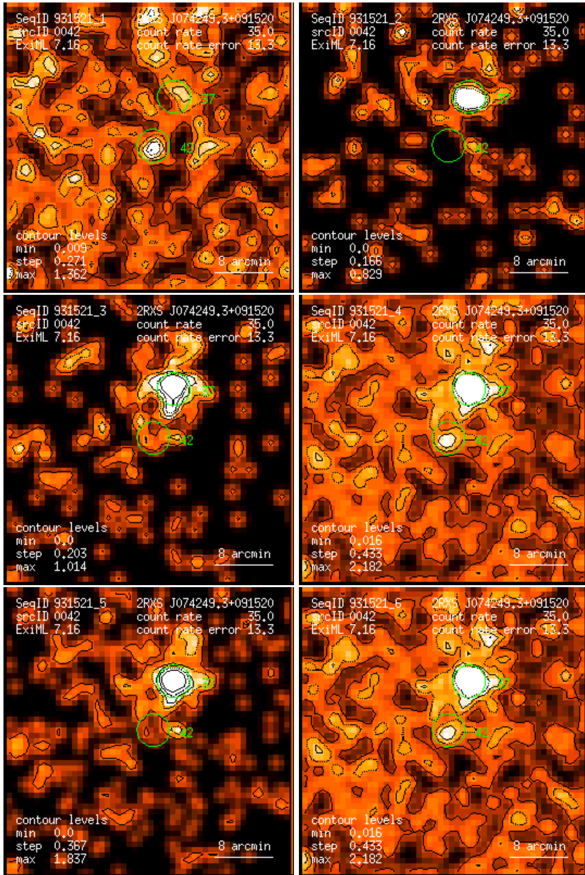
Figure 42: RASS 931521: detection 0042: band rate images, Gaussian filter: (1) PSPC channels 11 – 41, (2) 52 – 90, (3) 91 – 201, (4) 11 – 235, (5) 52 – 201, (6) 11 – 201. Broad band rates in counts/ks. Band rate contour levels in counts/ks/arcmin 2 .
