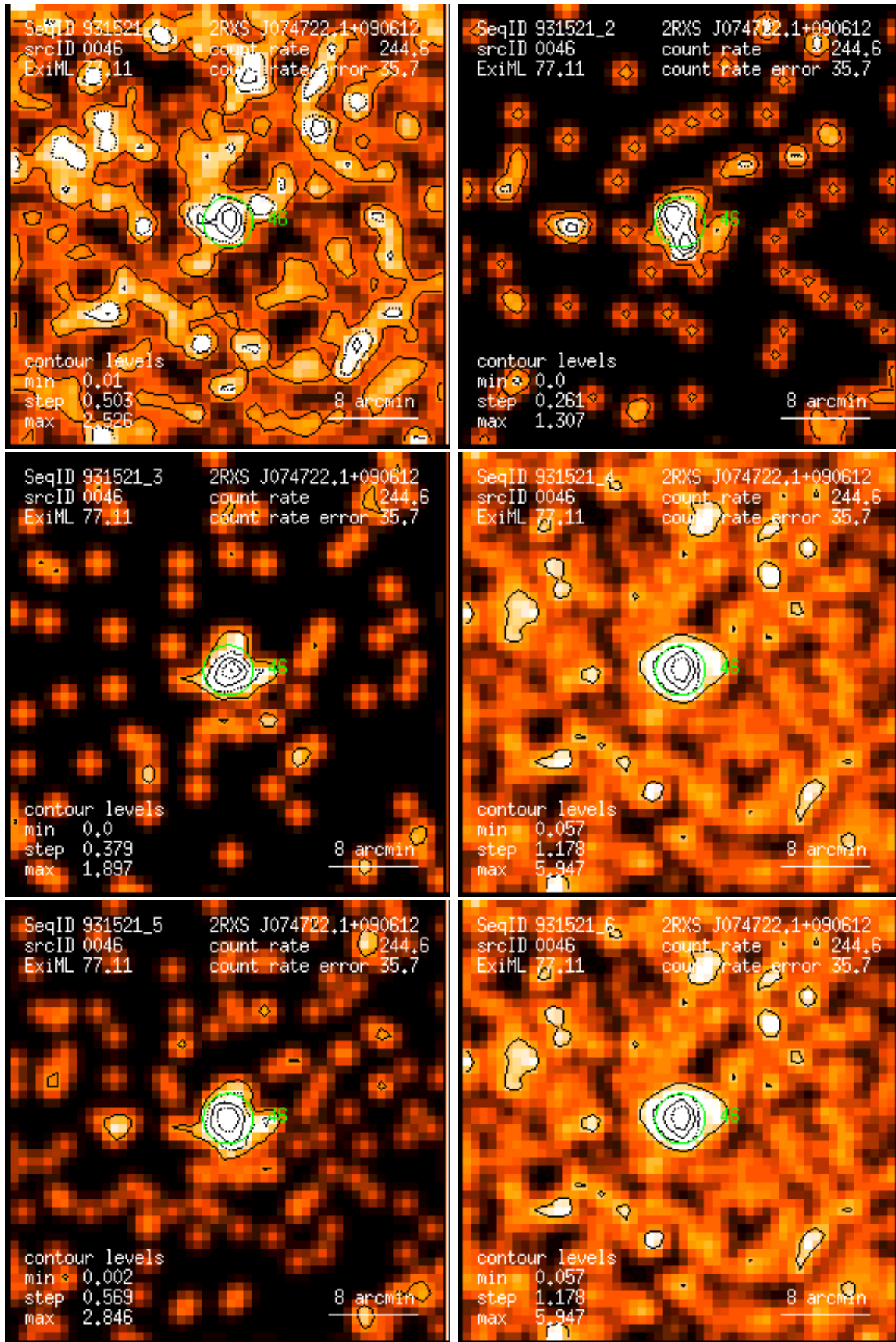
Figure 46: RASS 931521: detection 0046: band rate images, Gaussian filter: (1) PSPC channels 11 – 41, (2) 52 – 90, (3) 91 – 201, (4) 11 – 235, (5) 52 – 201, (6) 11 – 201. Broad band rates in counts/ks. Band rate contour levels in counts/ks/arcmin 2 .
