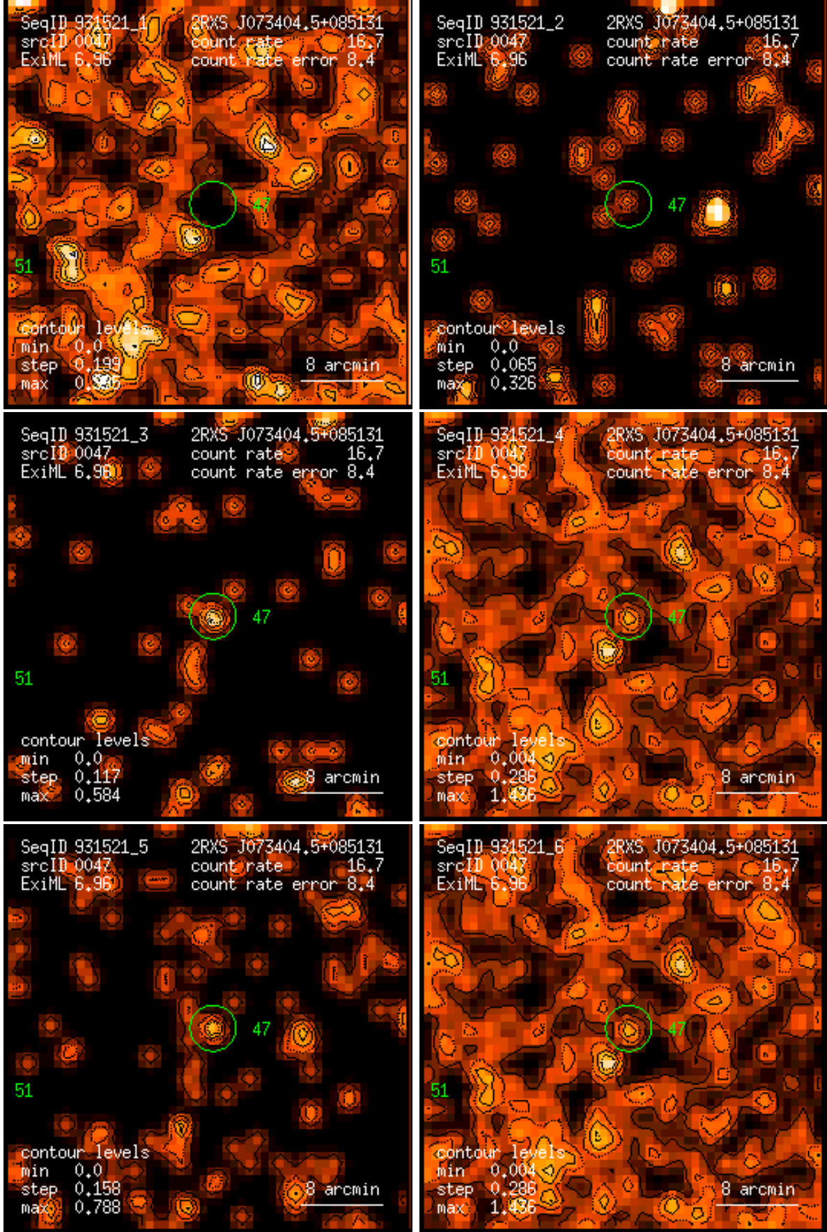
Figure 47: RASS 931521: detection 0047: band rate images, Gaussian filter: (1) PSPC channels 11 – 41, (2) 52 – 90, (3) 91 – 201, (4) 11 – 235, (5) 52 – 201, (6) 11 – 201. Broad band rates in counts/ks. Band rate contour levels in counts/ks/arcmin 2 .
